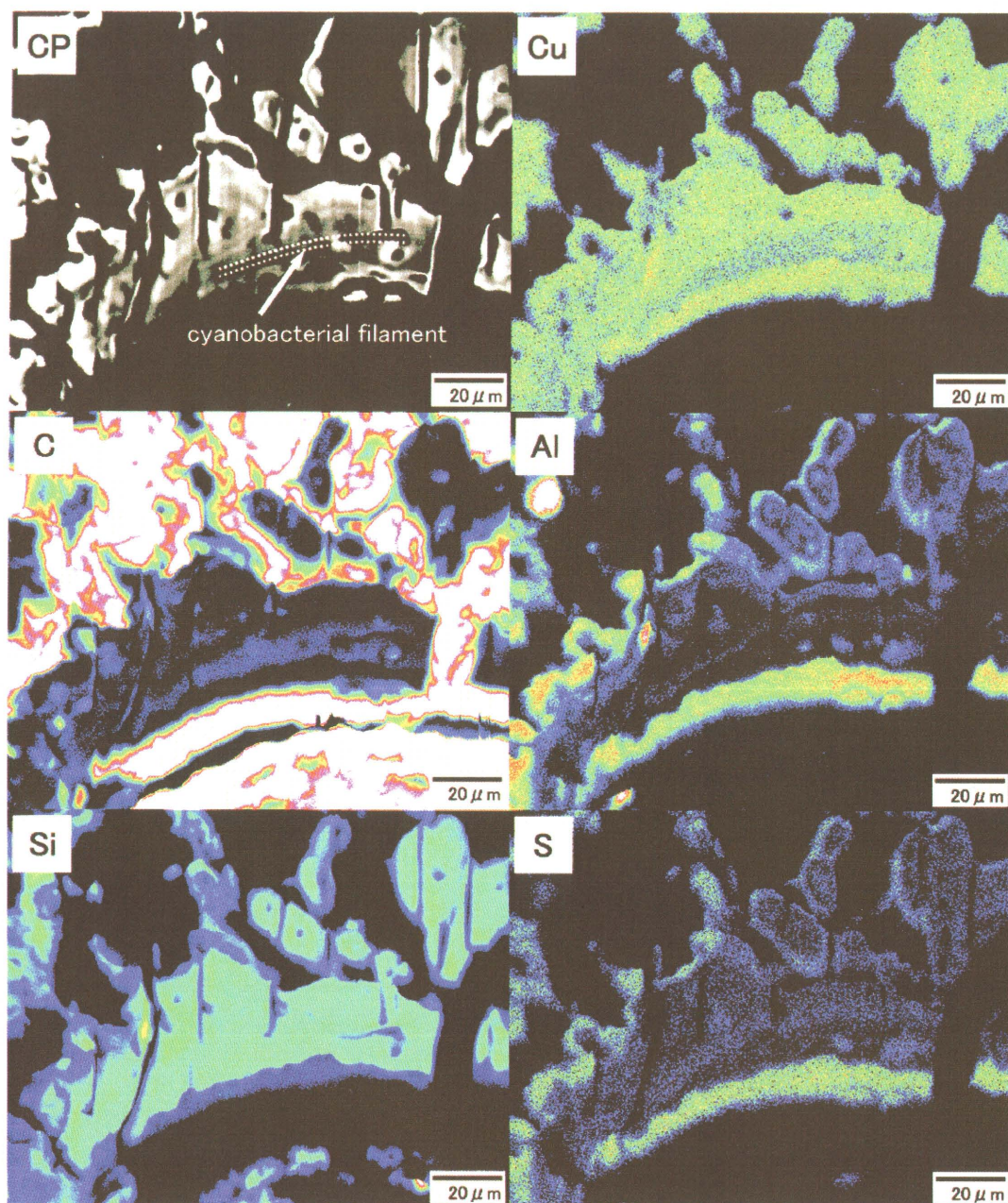
Fig. 25 EPMA color mapping of blue biomats reveals banded elemental distributions showing high Cu content at the light bands in BEI. Whereas, the Cu, Al and S are components of woodwardite showing high C and Si at the dark bands and around cyanobacterial filaments. Both Si and Cu are distributed at the same area.
