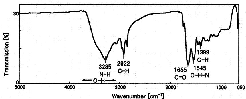
Fig. 5 FT-IR spectrum of green biomats indicating the presence of organic substance in the grain, showing 3700-3100 cm^{-1} (O-H stretch), 3285 cm^{-1} (N-H stretch), 2922 cm^{-1} (C-H stretch), 1655 cm^{-1} (C=O stretch), 1545 cm^{-1} (C-N-H stretch) and 1399 cm^{-1} (C-H stretch).
