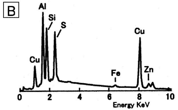
Fig. 9 Secondary electron images (A) and EDX spectrum (B) of green biomats showing the teardrop-shaped sheath and numerous filamentous cyanobacteria. Sheaths aggregate together with cyanobacteria and other grains. Sheaths consist mainly of Al, Si, S, Cu and Zn with the trace of Fe (B).
