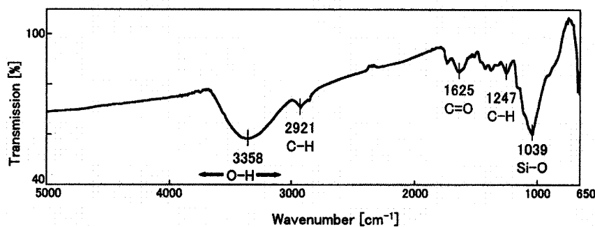
Fig. 17 FT-IR spectrum of blue biomats indicating the presence of organic substance in the grain, shows the bands at 3700-3100 cm^{-1} (O-H stretch), 2921 cm^{-1} (C-H stretch), 1625 cm^{-1} (C=O stretch), 1247 cm^{-1} (C-H stretch) and 1039 cm^{-1} (Si-O stretch).
