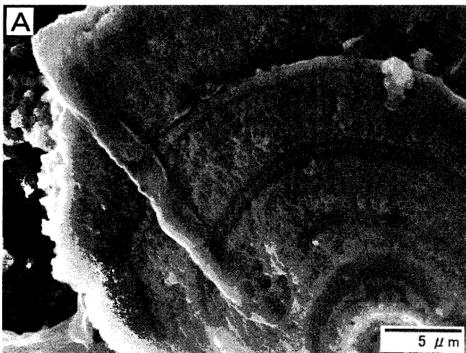
Fig. 10 SEM images of green biomats in sectioned sample recognize the lamina span corresponding to the length of the cells consisting of cyanobacterial filament (A: SEI, B: BEI).
