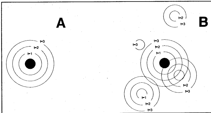
Fig. 1. Schematic representation of range spread between successive generations. The black dot represents the initial range at time 0. A. Spread according to Skellam's [26] diffusion model; B. Spread predicted using a stratified dispersal model.
