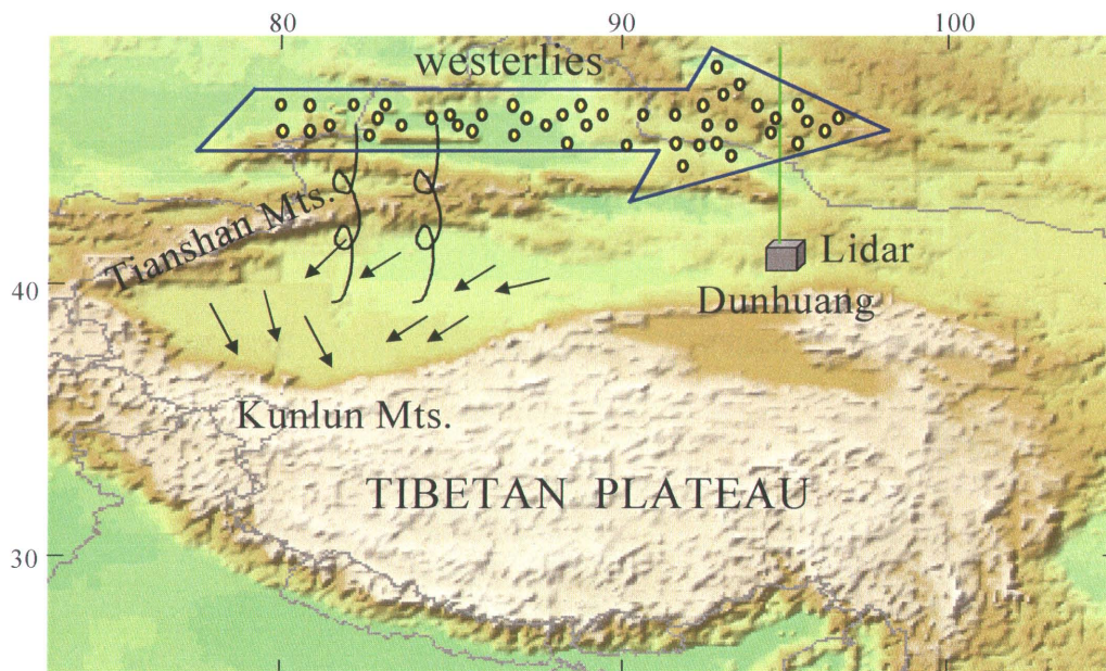
Fig.8 Schematic picture describing wind system and dust particle transports. Dominant surface wind is easterly (or northeasterly) at an elevation <math>< 5\text{km}</math>, and westerly at an elevation >math>> 5\text{km}</math>.
