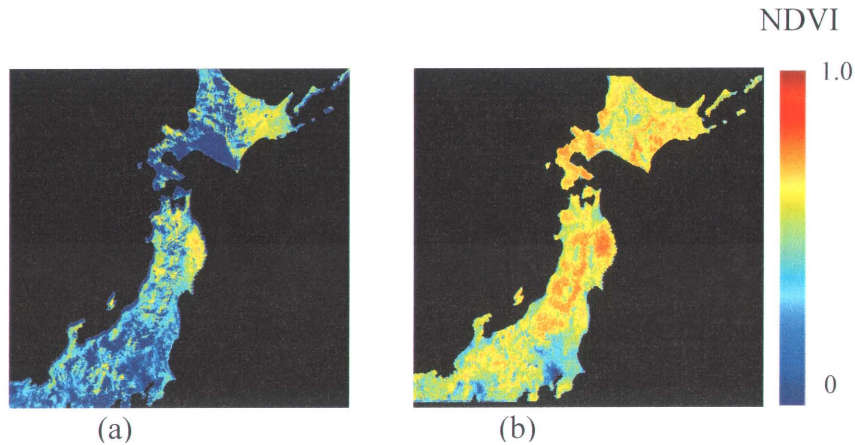
Fig. 12. (a) Daily NDVI image calculated from NOAA AVHRR dataset of 24 July 2004. (b) Monthly NDVI composite image of July 2004.
