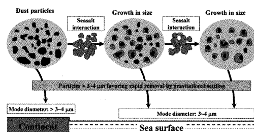
Figure1. Diagram of the dispersion and deposition of dust particles during their long-range transport in the marine boundary layer.
