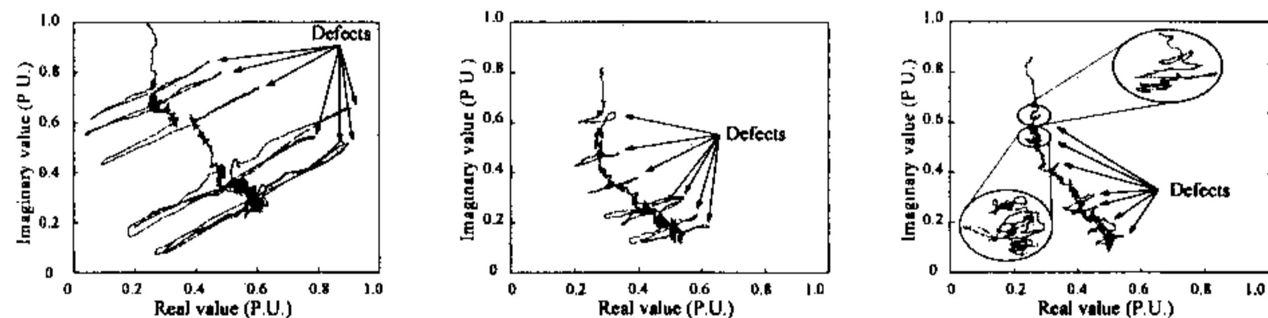
(a) 135 \mu\text{m} lift-off height (b) 185 \mu\text{m} lift-off height (c) 235 \mu\text{m} lift-off height Fig. 7. Effect of lift-off height to the ECT signal variation
