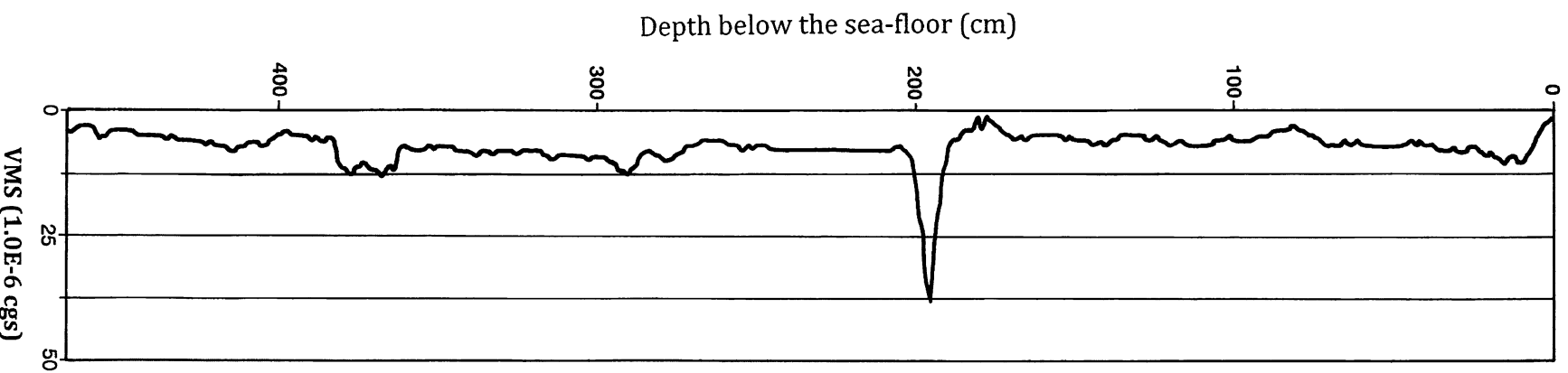
Fig. 3 Volume magnetic susceptibility of the core KT99-14 P-11.
