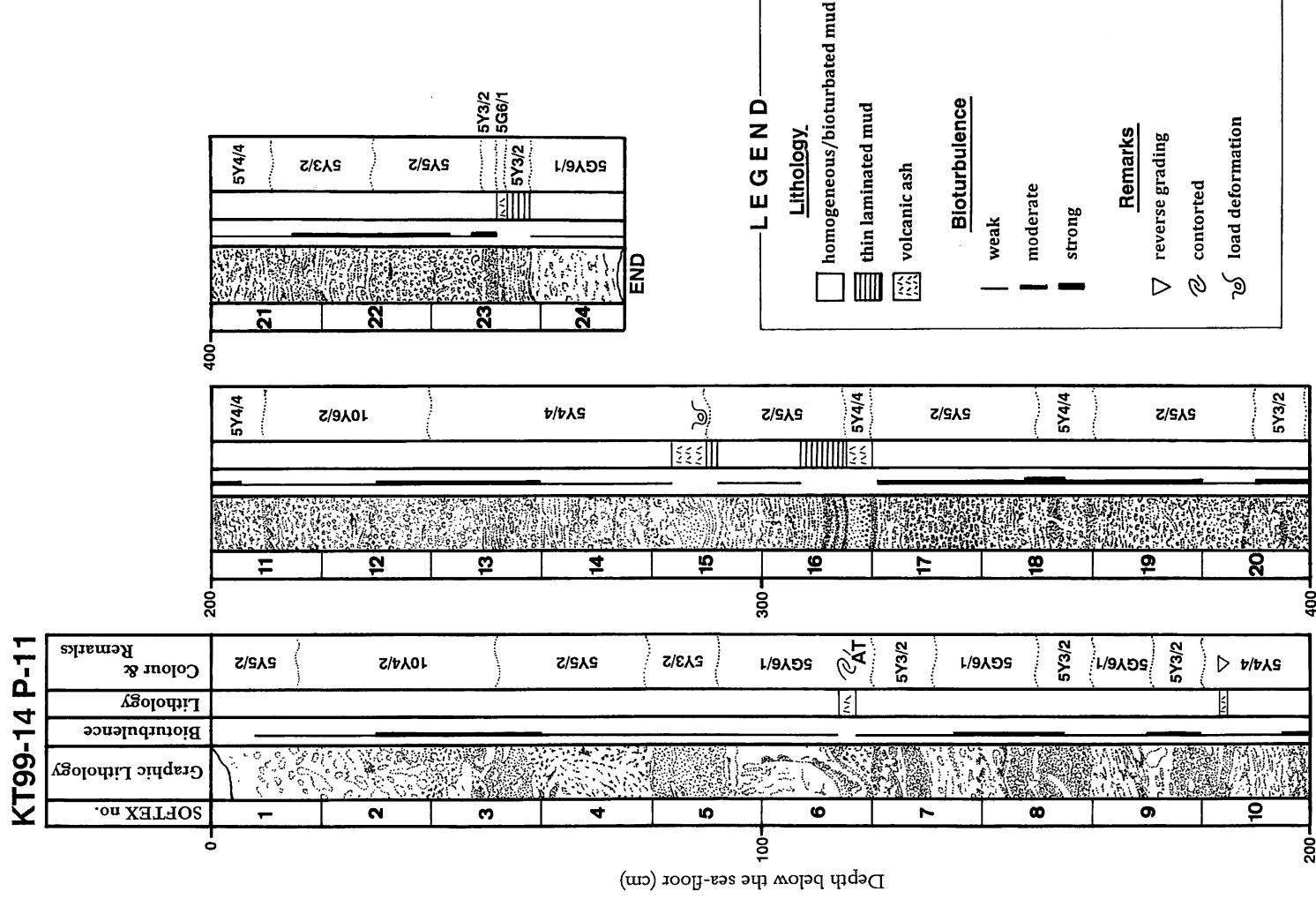
Fig. 2 Graphic descriptions of the core KT99-14 P-11.
