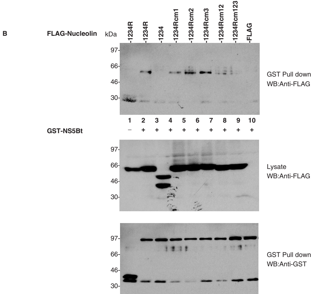
Fig. 6. Interaction of NS5Bt with clustered mutants (cm) of nucleolin 1234R. COS cells were transiently co-transfected with plasmids expressing FLAG-nucleolin 1234R proteins and GST protein alone or GST-NS5Bt protein. (A) Schematic diagrams of wild-type nucleolin and clustered mutants. This figure shows a series of clustered mutants. All of arginine and phenylalanine residues in three regions within nucleolin GAR domain were substituted to alanines in each mutants. (B) GST pull-down assay and Western blot analysis were carried out with anti FLAG antibody and anti GST antibody. Upper panel is output of FLAG-nucleolin 1234R proteins. Co-precipitants on
