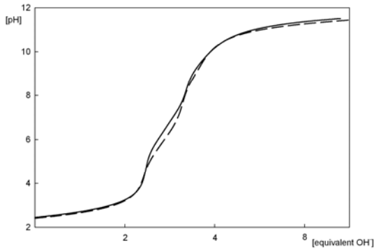
Figure 3 Titration curves of IP and IP/Spd systems. c_{\text{IP}}=c_{\text{Spd}}=0.001\text{M} — experimental titration curve of IP - - - experimental titration curve of the IP/Spd system
