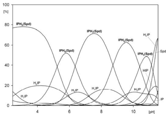
Figure 4 Calculated distribution diagram for IP/Spd system. Percentage refers to total IP; [\text{IP}]=0.001\text{M} , [\text{Spd}]=0.001\text{M}
