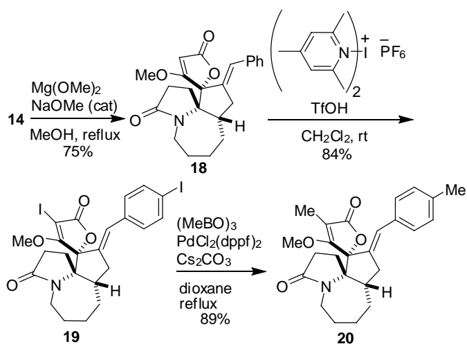
Scheme 5. Synthesis of 20 .
