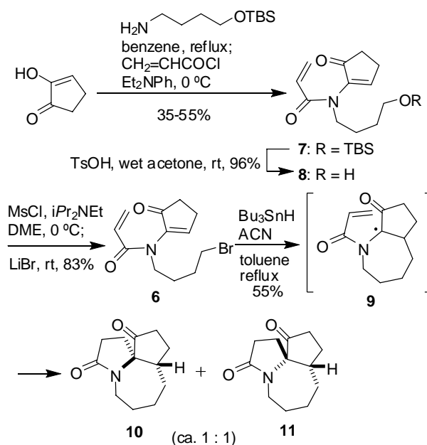
Scheme 2. Synthesis and radical cyclization of 6 .
