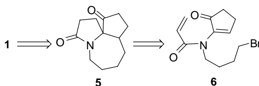
Scheme 1. Retrosynthetic analysis.
