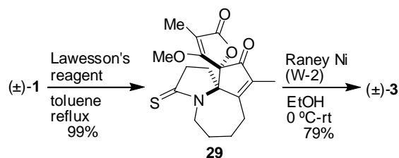
Scheme 10. Synthesis of (±)-3.
