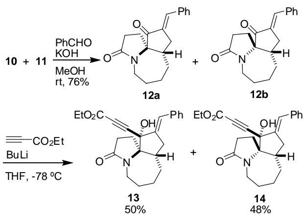
Scheme 3. Synthesis of 13 and 14 .
