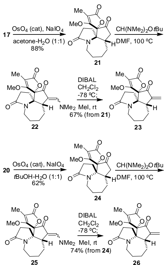
Scheme 6. Synthesis of 23 and 26
