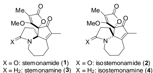
Figure 1. Stemonamide and related alkaloids.
