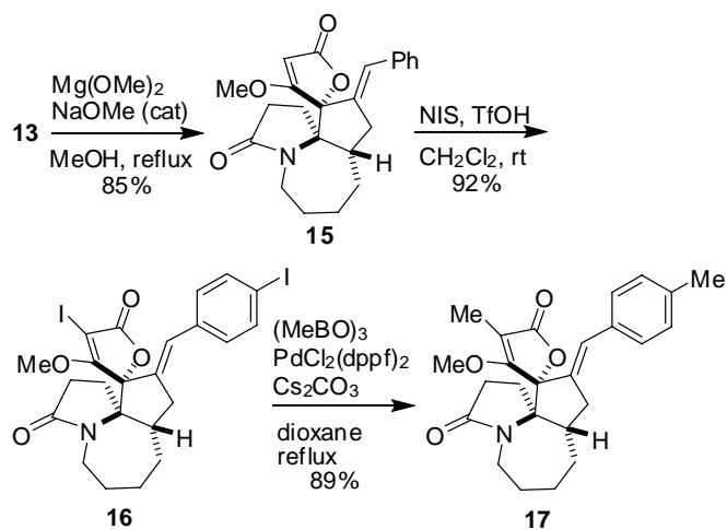
Scheme 4. Synthesis of 17 .
