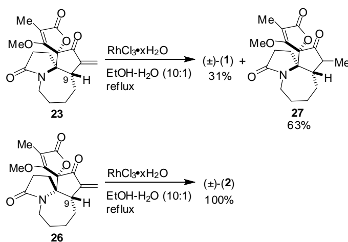
Scheme 7. Synthesis of (±)- 1 and (±)- 2 .
