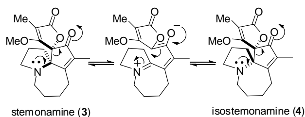
Scheme 9. Equilibrium between 3 and 4 .
