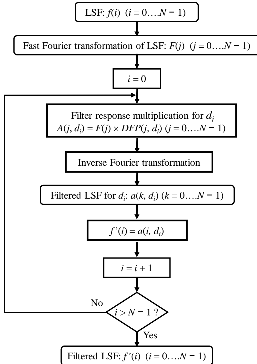
Fig. 5 Variable filtering processing procedure
