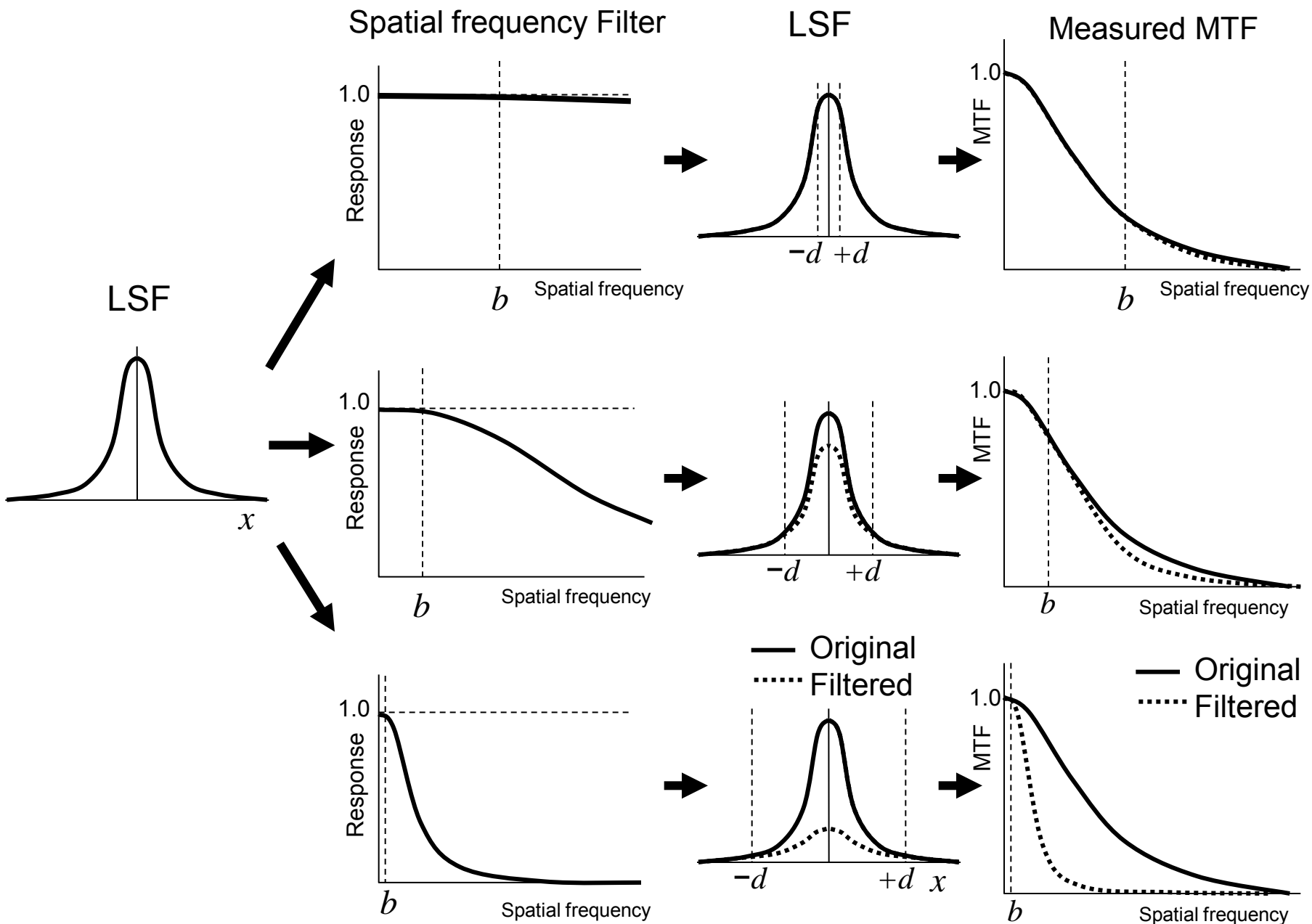
Fig. 3 Relationship between the boundary frequency b in the presampled MTF and distance d in the LSF. The LSF tails outside of d are maintained when the frequency region below b (= 1/2d) is not filtered
