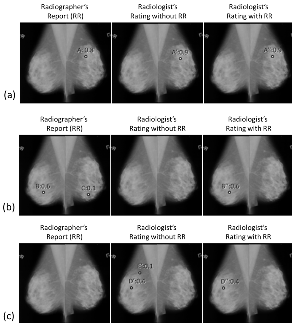
Fig. 2 Example of selections of responses for simulated radiologist's rating utilizing a radiographer's report
