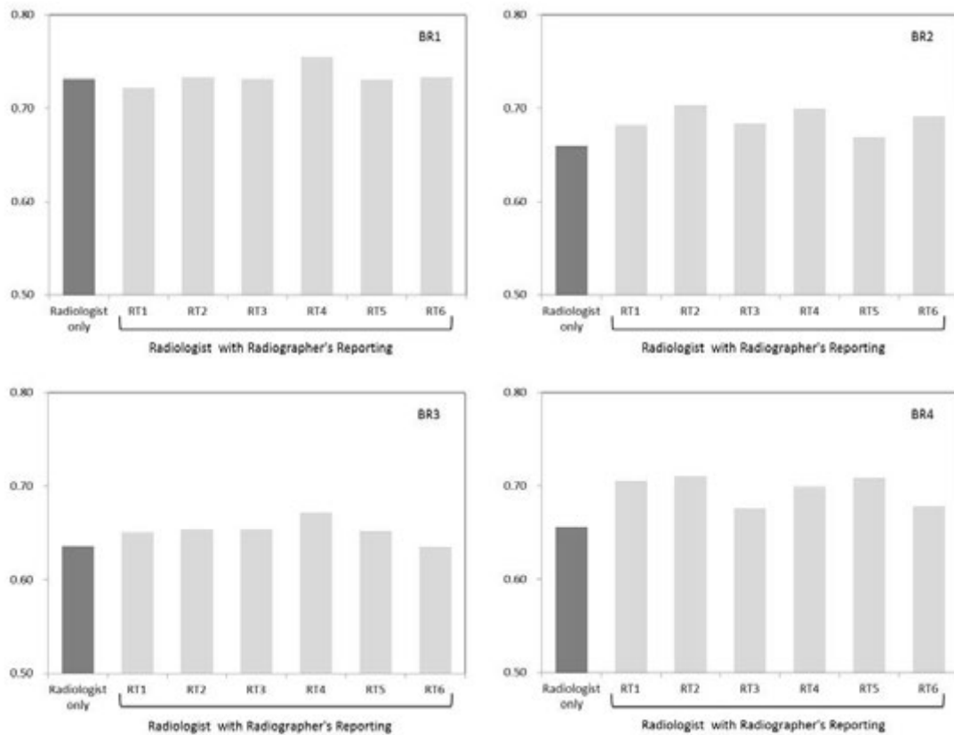
Fig. 4 Change of the figure of merit (FOM) of radiologists' performances with and without each of 6 radiographers' report
