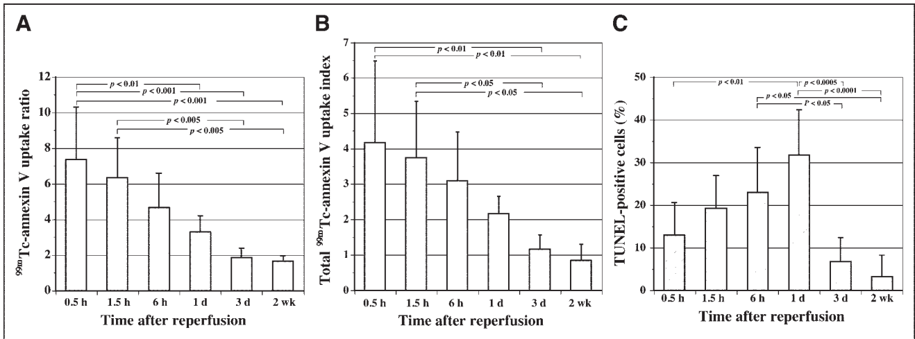
FIGURE 3. (A) Time course of ^{99m}\text{Tc} -annexin V uptake ratio in the apoptotic area after ischemia and reperfusion. Time after reperfusion indicates the time of ^{99m}\text{Tc} -annexin V injection. ^{99m}\text{Tc} -Annexin V uptake ratio was highest shortly after reperfusion. (B) Time course of total ^{99m}\text{Tc} -annexin V uptake index, showing results similar to those for ^{99m}\text{Tc} -annexin V uptake ratio. Total uptake was highest at 30 min after reperfusion and decreased with time over the next 3 d. (C) Time course of the percentage of TUNEL stain–positive cardiomyocytes after reperfusion. Time after reperfusion indicates the time of ^{99m}\text{Tc} -annexin V injection. TUNEL positivity increased up to 1 d after reperfusion and then significantly declined at 3 d after reperfusion.
