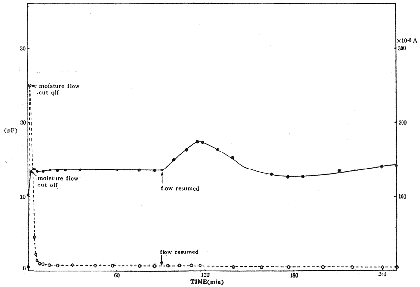
Fig. 6 The result of a simultaneous measurement of the capacitance and conductivity when moisture flow was cut off at the time of peak of the conductivity. (soda lime glass)
