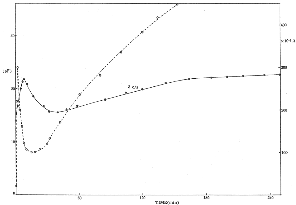
Fig. 16 The result of a simultaneous measurement of the capacitance and conductivity. (calcined diatomaceous earth)
