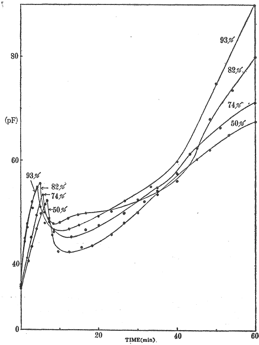
Fig. 20 Changes of capacitance at several relative humidities. (calcined diatomaceous earth)
