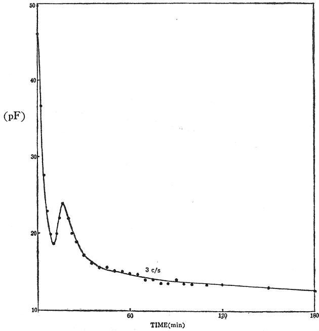
Fig. 14 Capacitance changes when a mica plate with adsorbed water was slowly dried. (mica)
