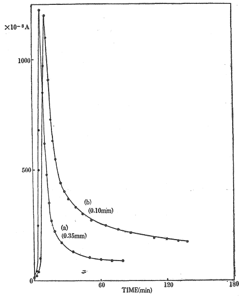
Fig. 3 Surface conductivity changes during moisture adsorption. (soda lime glass)
