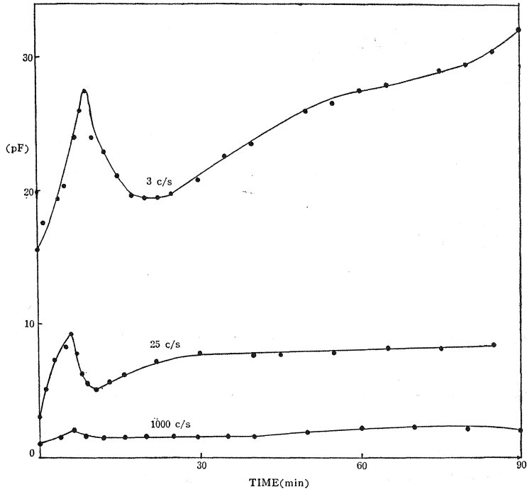
Fig. 13 Capacitance changes during moisture (82% relative humidity) adsorption at the frequencies indicated. (mica)
