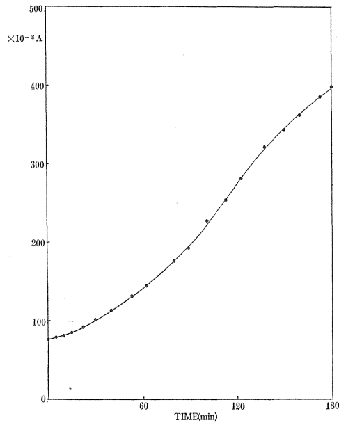
Fig. 9 Surface conductivity changes during moisture adsorption. (soda lime glass)
