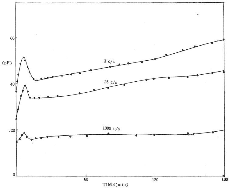
Fig. 10 Capacitance changes during moisture adsorption measured at the frequencies indicated. (mica)
