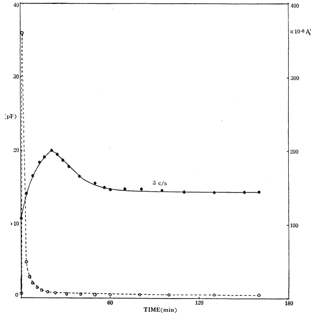
Fig. 5 The result of a simultaneous measurement of the capacitance and conductivity. (soda lime glass) Solid curve : Capacitance, Broken curve : Conductivity.
