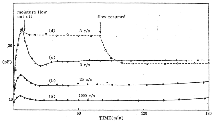
Fig. 1 Capacitance changes during moisture adsorption measured at the frequencies indicated. (soda lime glass)
