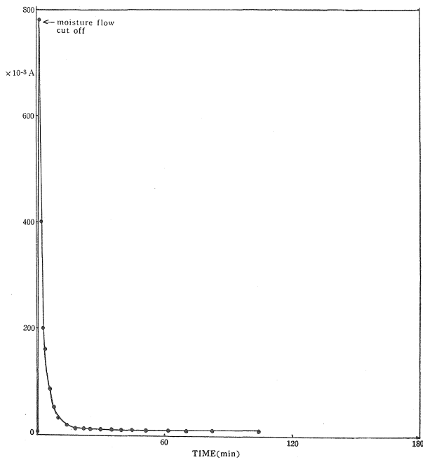
Fig. 12 Surface conductivity changes when moisture flow was cut off at the time of the peak. (mica)
