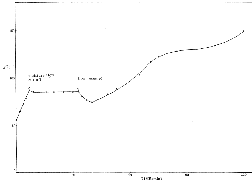
Fig. 21 Capacitance changes when moisture flow was cut off and set up again. (calcined diatomaceous earth)
