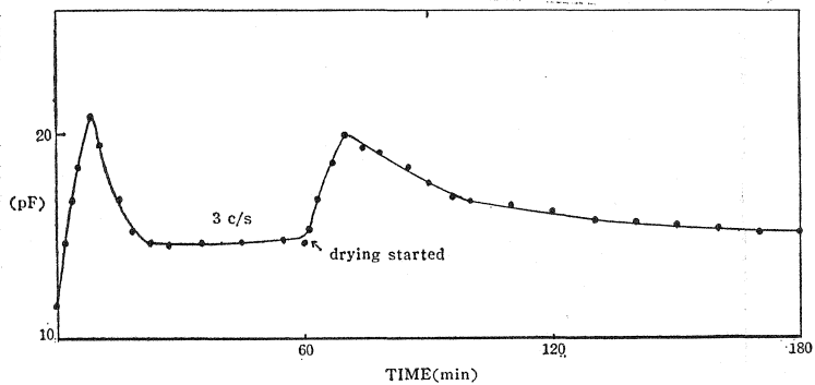
Fig. 2 Capacitance changes when a glass plate with adsorbed water was slowly dried. (soda lime glass)
