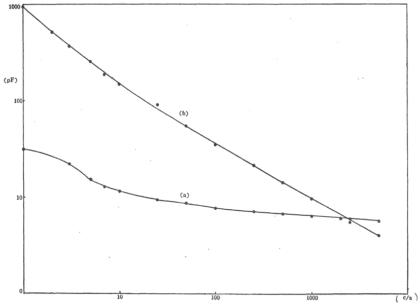
Fig. 19 Frequency dependences of the capacitance. (calcined diatomaceous earth)
