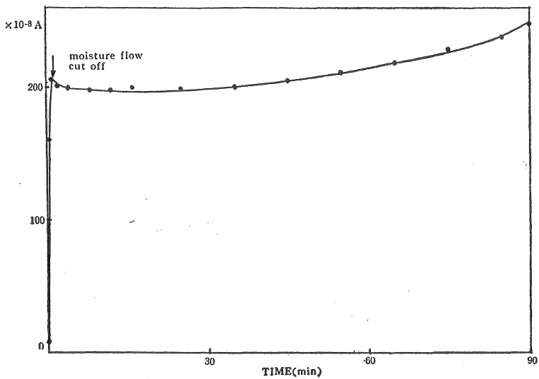
Fig. 4 Surface conductivity changes when moisture flow was cut off before it reached the peak. (soda lime glass)
