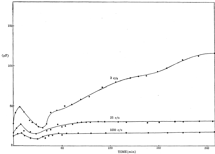
Fig. 17 Capacitance changes during moisture adsorption at the frequencies indicated. (pinhole of the leak cock is 1.5mm in diameter). (cacid diatomaceous earth)
