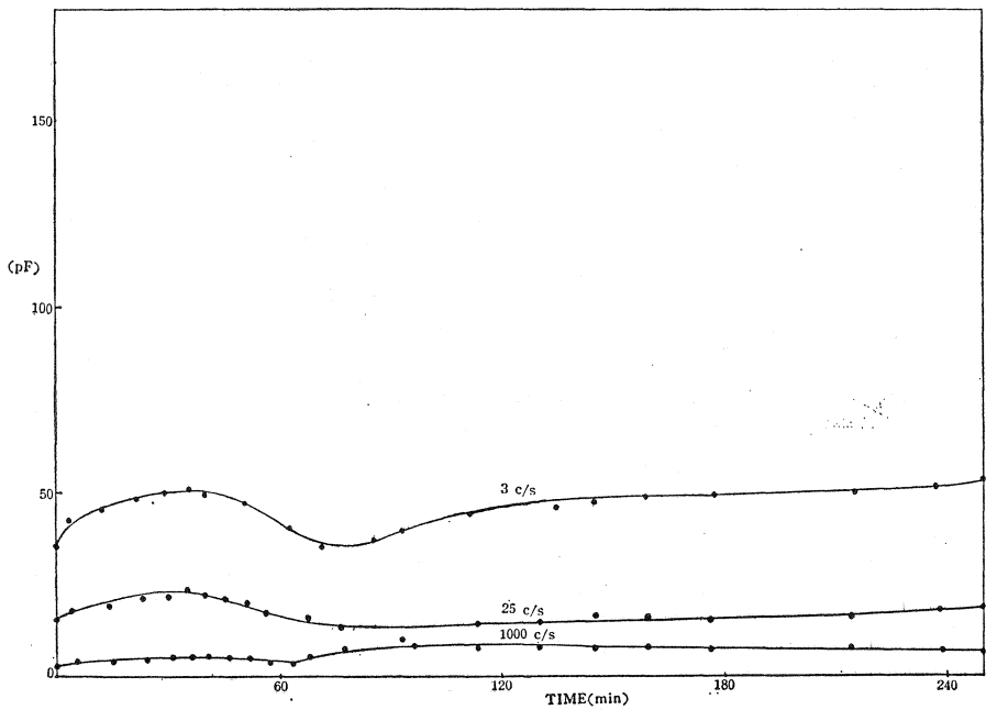
Fig. 18 Capacitance changes during moisture adsorption at the frequencies indicated (pinhole of the leak cock is 0,3mm in diameter). (calcined diatomaceous earth)
