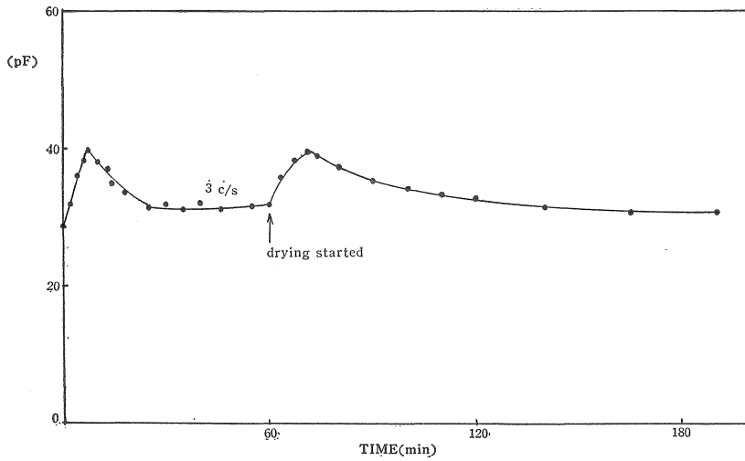
Fig. 11 Capacitance changes when a mica plate with adsorbed water was slowly dried. (mica)
