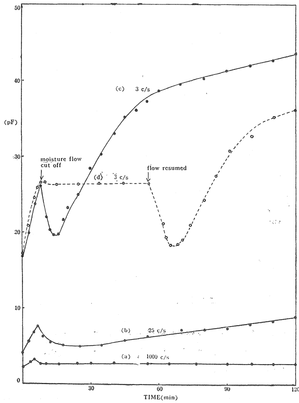
Fig. 7 Capacitance changes during moisture adsorption measured at the frequencies indicated. (soda lime glass)
