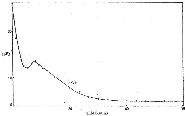
Fig. 8 Capacitance changes when a glass plate with adsorbed water was slowly dried. (soda lime glass)
