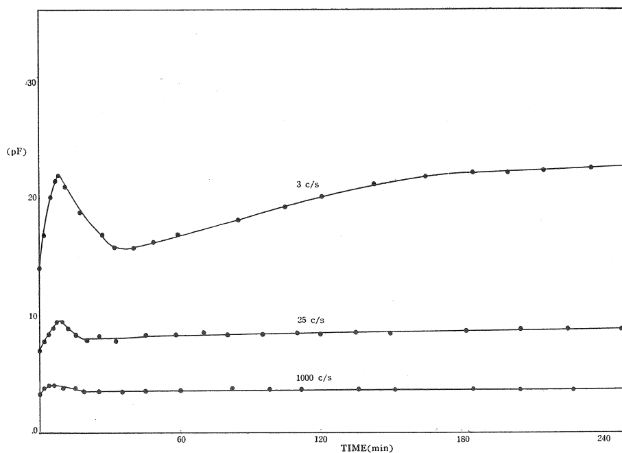
Fig. 15 Capacitance changes during moisture adsorption at the frequencies indicated. (calcined diatomaceous earth)
