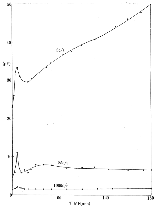
Fig. 22 Capacitance changes during moisture adsorption measured at the frequencies indicated. (filter paper)
