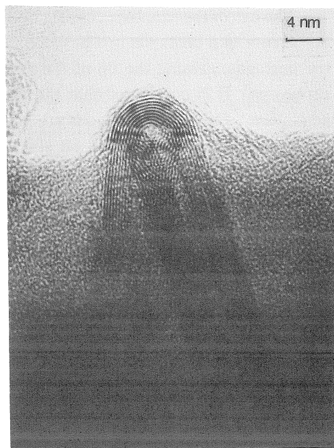
Fig. 5. Electron micrograph of two carbon nanotubes that overlap each other at the end of it. Individual dark line corresponds to the graphite sheets separated by 0.34 nm.
