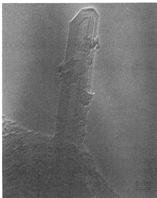
Fig. 3. (b) Close up micrograph of (a). The graphite layer structure \{002\} can be observed.
