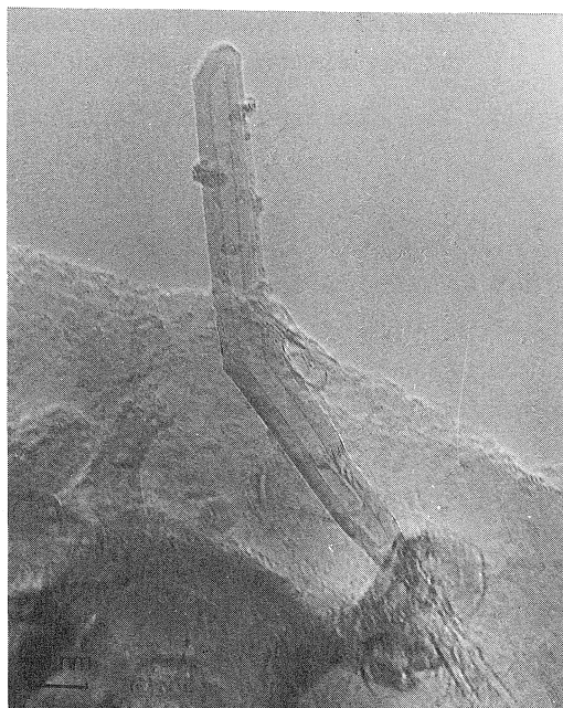
Fig. 3. (a) Electron micrograph showing carbon nanotube consisting of two caps. This nanotube was formed on the carbon string and is bending in the middle section.
