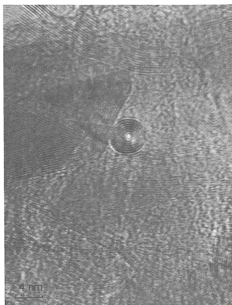
Fig. 7. Electron micrograph of a near spherical nanoparticle. This nanoparticle is 5.1 nm in diameter. The minimum circle in the center is approximately 0.7 nm in diameter.
