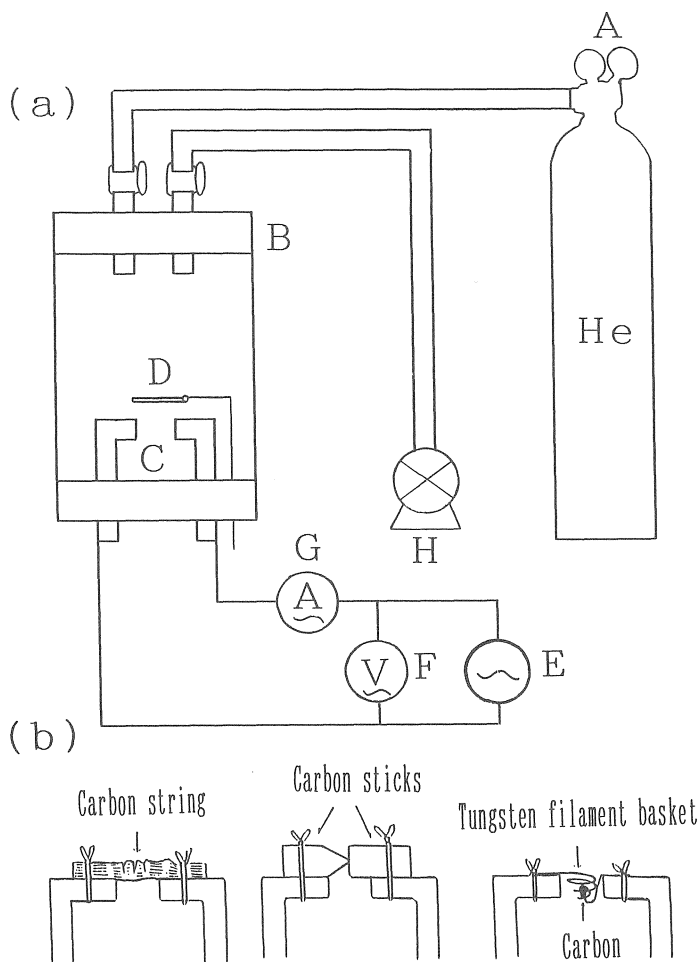
Fig. 2. (a) Schematic diagram of a.c. arc-discharge evaporation method apparatus. A, pressure gauge; B, reaction chamber; C, copper rod; D, substrate; E, slide rheostat; F, voltmeter; G, ammeter; H, rotary pump.
