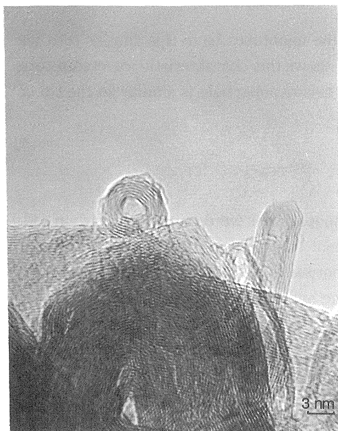
Fig. 6. Electron micrograph of a near spherical nanoparticle with a hollow found on the carbon string.
