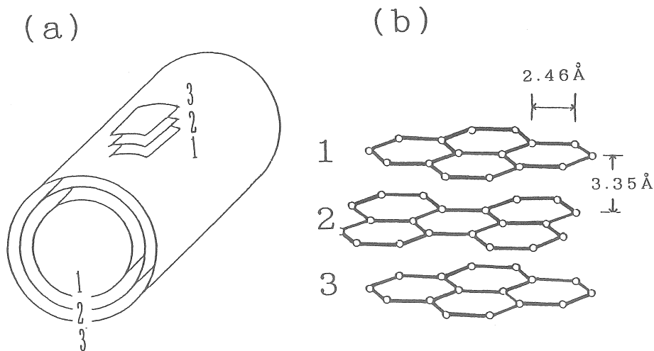
Fig. 1. (a) Schematic diagram of the structural model of the carbon nanotube reported by Iijima (1991). The number corresponds to the rolling of graphite layers. (b) Schematic diagram of the three sheets of graphite.
