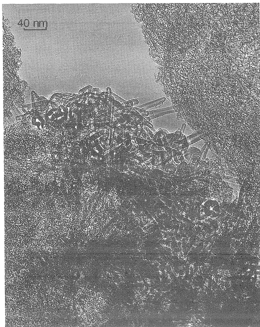
Fig. 4. Electron micrograph of carbon nanotubes and nanoparticles that were formed on the carbon string.
