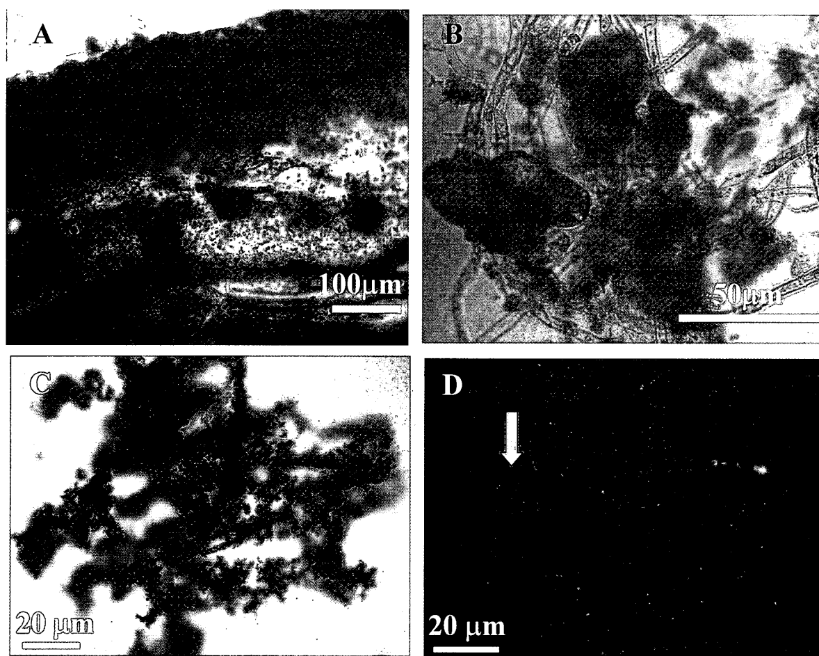
Fig. 17. Micrographs of green biomats collected from V5 hot springs. Thin section of green biomats (A). Calcite balls array parallel to the layering of biomats. Calcite balls attached on fibrous algae in the biomats (B). Optical micrograph of brown microbial mats at the Vilyuchinskie hot springs showing the filamentous mineral particles (C). Variety of bacteria associated with the minerals (an arrow) is inferred by intense green luminescence under epifluorescence mode (D).
