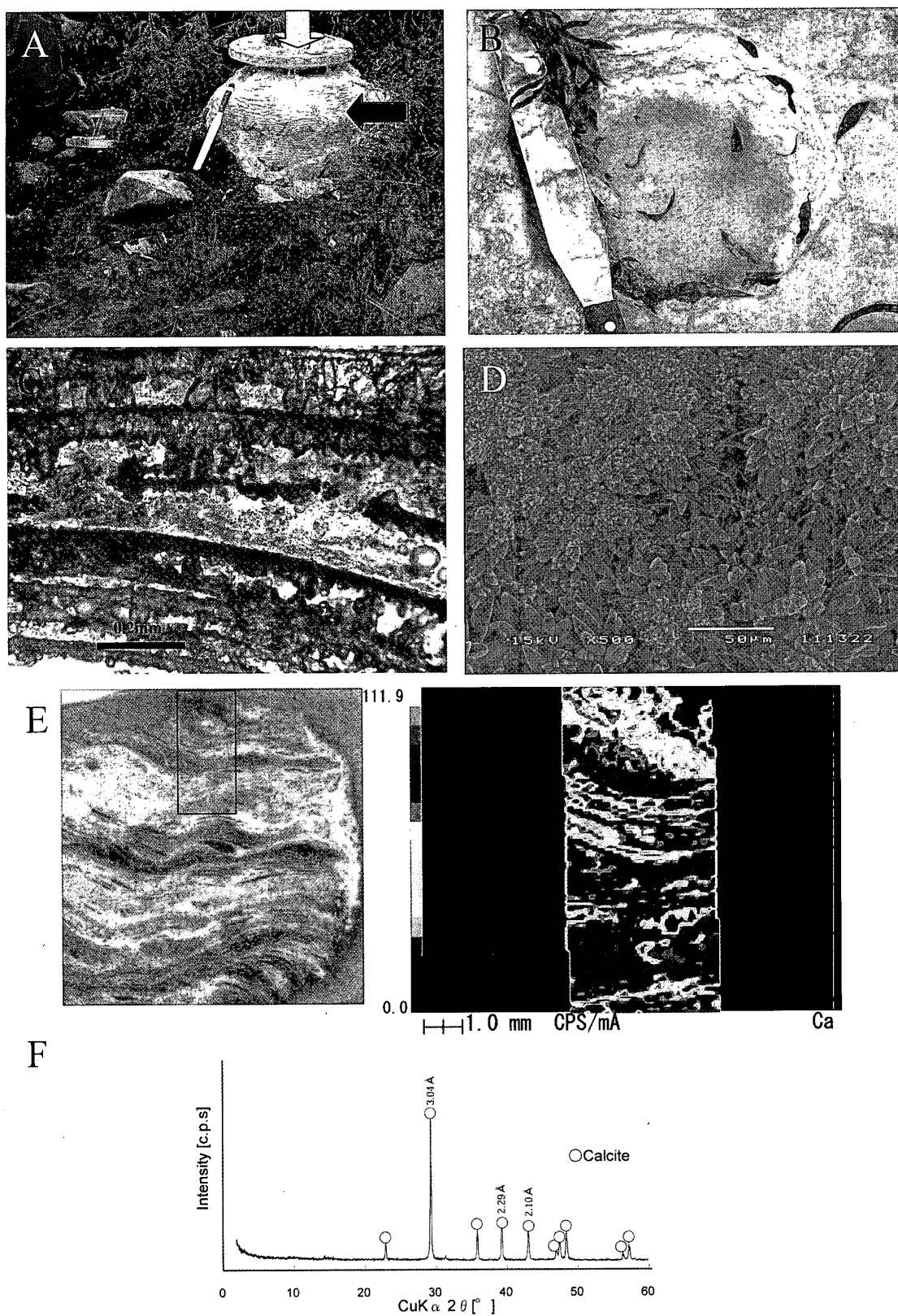
Fig. 15. Field views of source of well in Vilyuchinsk-3 hot springs in Southern Kamchatka (A). Micrograph of thin section of travertine collected at the middle part of the well (pointed by red an arrow in A) (B). Calcite thin film formed on the pit of well (pointed by blue an arrow in A) (C). SEM image of the calcite thin films (D). ED-XRF elemental map showing layered Ca distribution in the travertine shown in B (E). Analyzed area is indicated by red box in the photograph left side of the elemental map (E). XRD patterns of the calcite thin films identified pure calcite (F).
