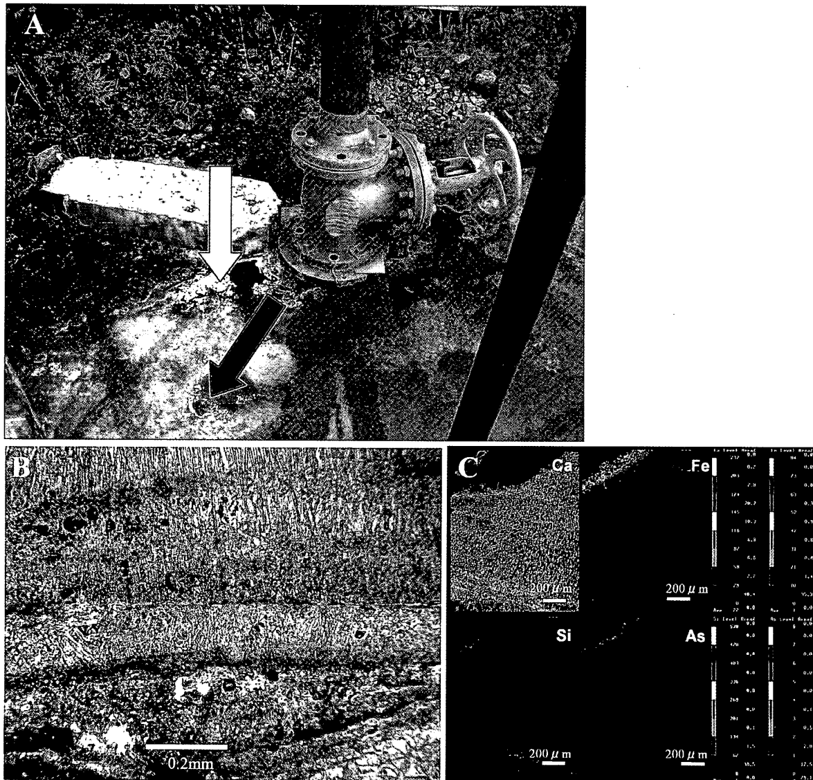
Fig. 14. Field view of water pump in Vilyuchinskies-2 hot springs in Southern Kamchatka (A). Travertine (blue an arrow) and calcite films (red an arrow) are formed. Micrograph of thin section of travertine collected from the point indicated by blue an arrow in A (B). EPMA chemical composition maps of the travertine (blue an arrow) showed concentration of Fe, As, and Si on the surface of travertine (C).
