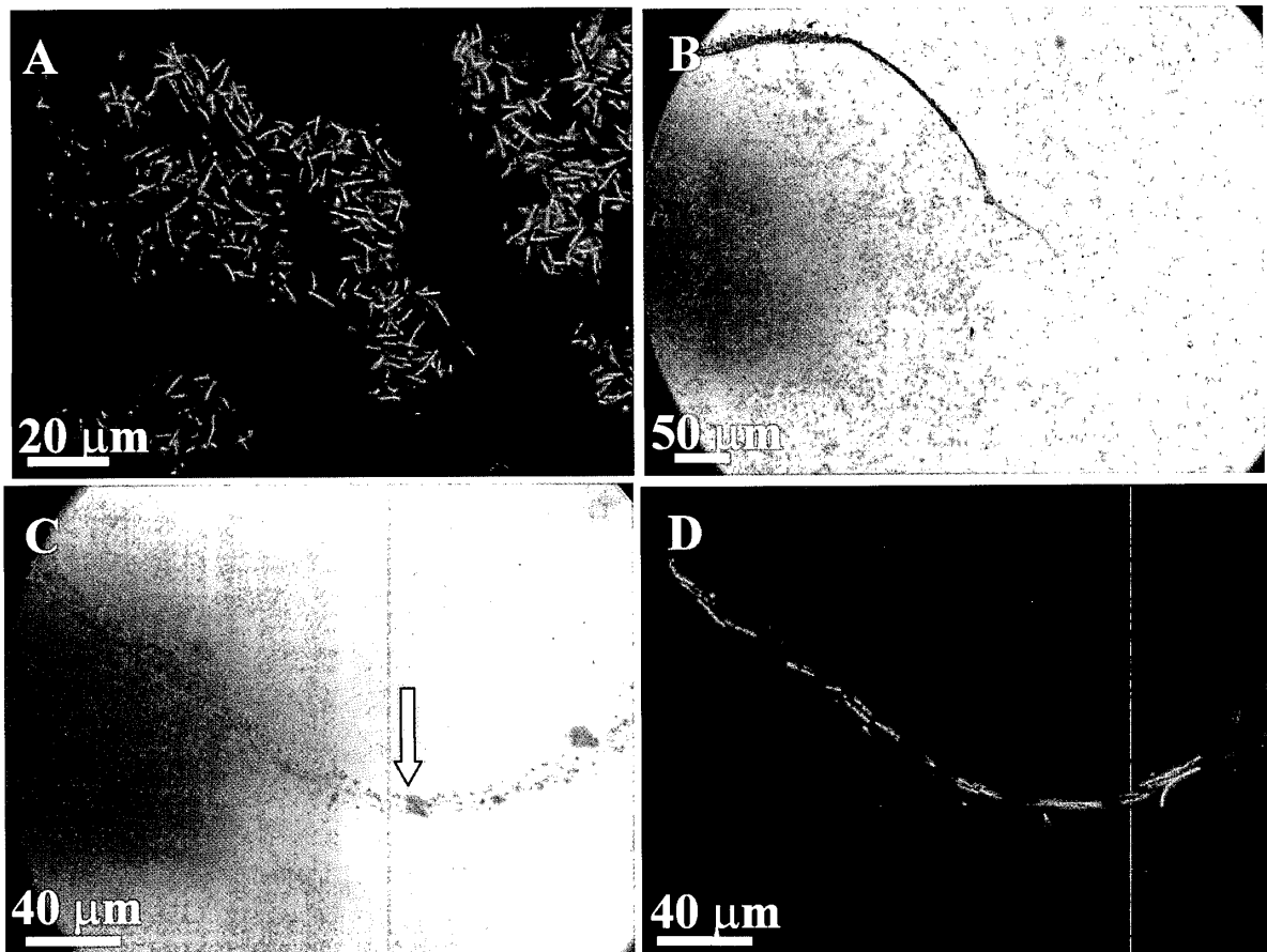
Fig. 13. Optical micrographs of white (A) and black (B, C and D) microbial mats collected from the Dachnye hot springs. Epifluorescence micrograph (A) shows long rods-shaped bacteria that are dominant in white bacterial mats. Optical images of the black filament (B, C and D) showing bacteria associated with mineral particles (an arrow).
