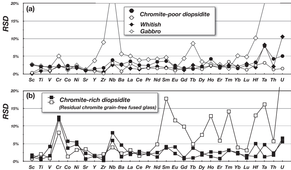
Figure 3. Precision of 3-spot LA-ICP-MS analytical data of the fused glass of studied samples. RSD is relative standard deviation ( 1\sigma ). (a) chromite-poor diopsidite (2 fused glass beads), whitish rock and gabbro samples. (b) chromite-rich diopsidite sample. 2 sets of 3-spot analyses were carried out on a bead of the single residual chromite grain-free fused glass (closed square). Open square indicates analytical data using a spot size of 30 \mu\text{m} (see text).
