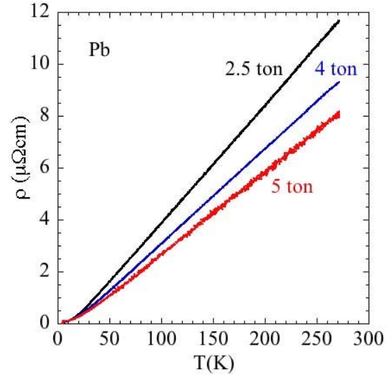
Figure 4. The electrical resistivity of lead as a function of temperature up to room temperature for several pressure loads.
