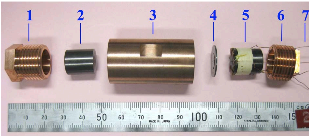
Figure 1. Photograph of the high-pressure cell: (1) upper screw, (2) upper anvil, (3) cylinder, (4) gasket, (5) lower anvil, (6) lower screw, (7) electrical leads. See the text for details.
