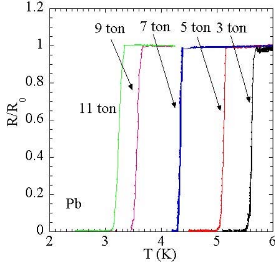
Figure 2. Temperature dependence of the relative electrical resistance of lead at various loads by using a clamp cell. R_0 is the resistance in the normal conducting state.
