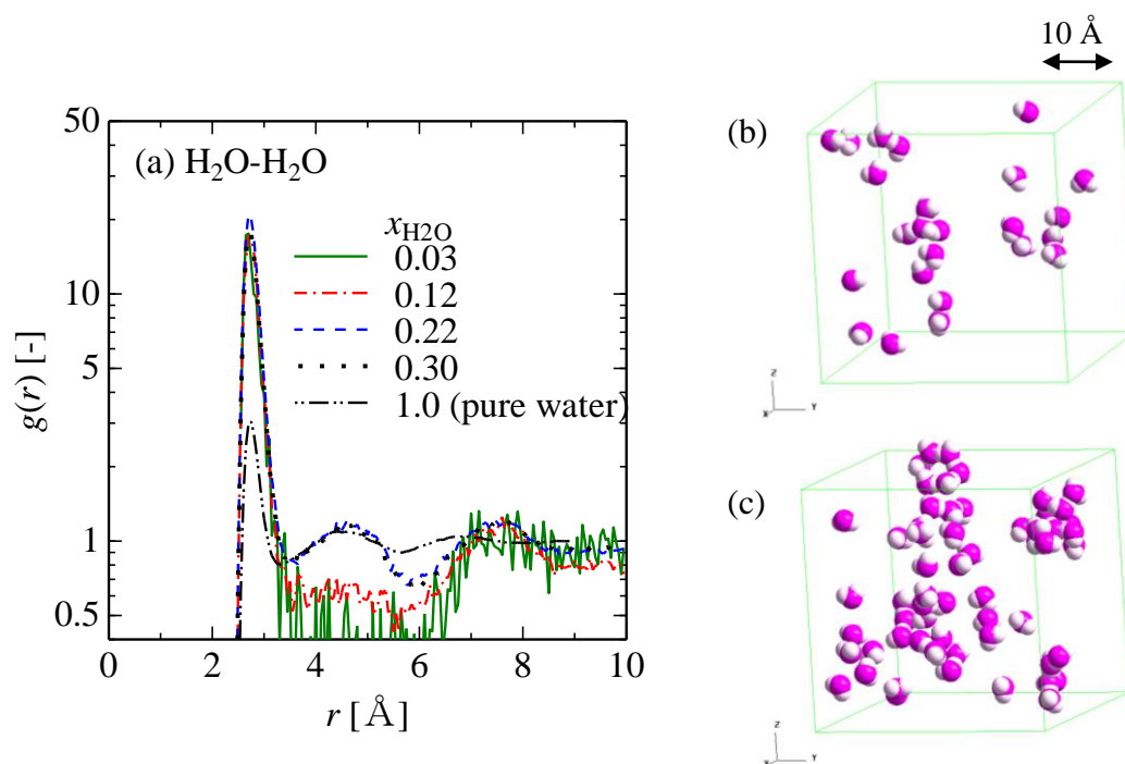
Figure 5 (a) Radial distribution function for H 2 O-H 2 O and water configuration ((b) x H2O =0.12, (c) x H2O =0.30, except for the
