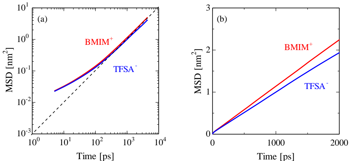
Figure 1 Mean square displacements of BMIM + and TFSA - molecules at 353 K
