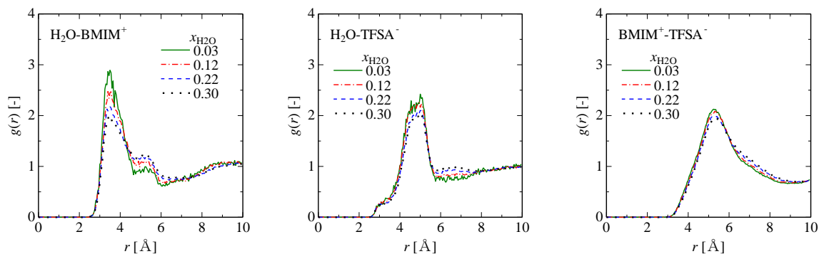
Figure 4 Radial distribution functions for H 2 O-BMIM + , H 2 O-TFSA - and BMIM + -TFSA - for the [BMIM][TFSA]/water
