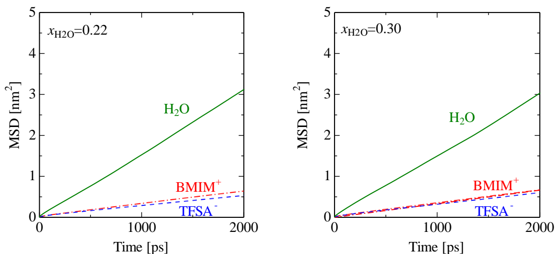
Figure 2 Mean square displacement of cation, anion, and water molecules for the [BMIM][TFSA]/water system
