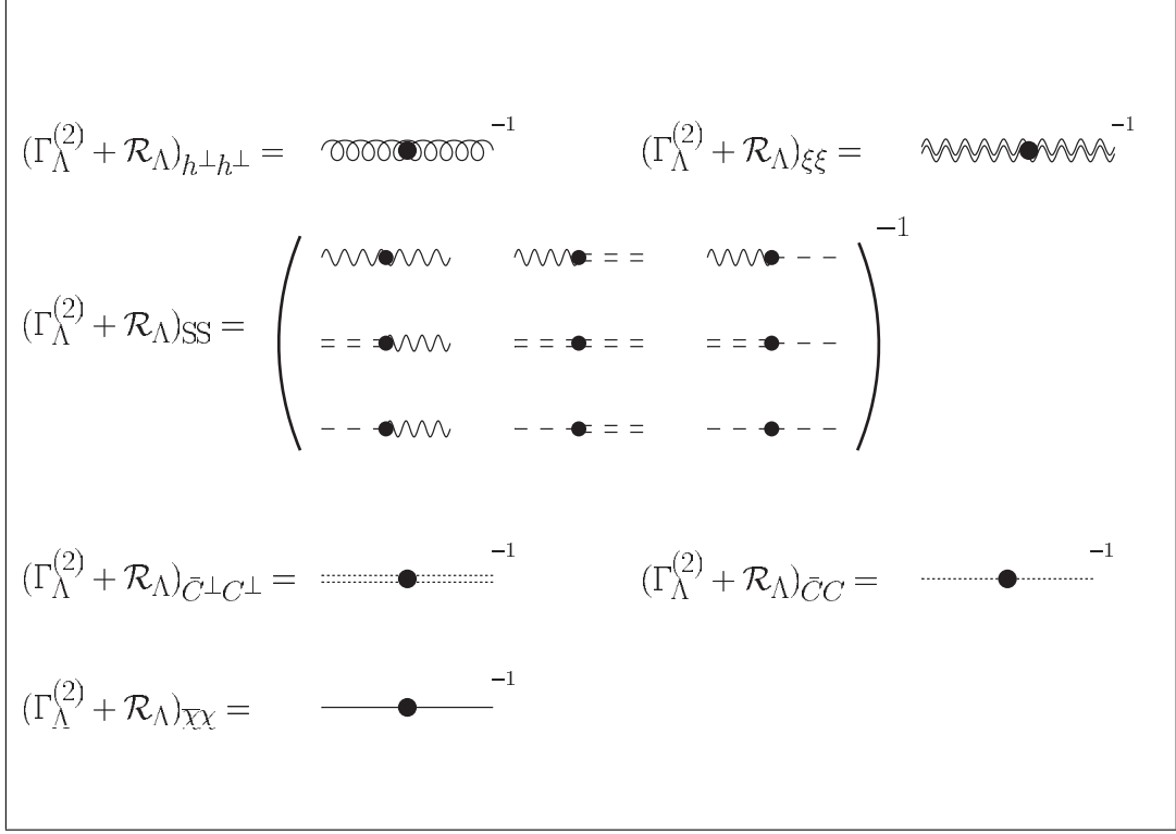
Figure 2: The propagators in the truncated effective action
