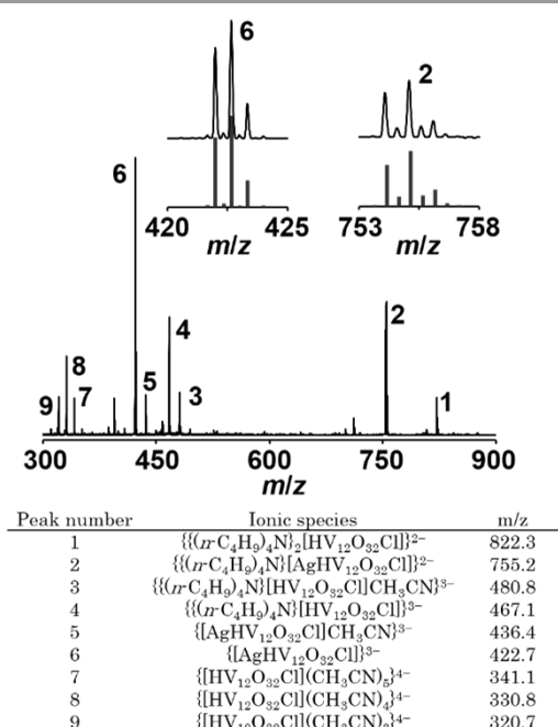
Fig. 6 ESI-MS spectrum of closed-V12' . The lines in the insets are the calculated patterns for \{[\text{Ag}[\text{HV}_{12}\text{O}_{32}(\text{Cl})]\}^{3-} ( m/z = 422.7 ) and \{((n-\text{C}_4\text{H}_9)_4\text{N})_3\text{Ag}[\text{HV}_{12}\text{O}_{32}(\text{Cl})]\}^{2-} ( m/z = 755.2 ). A table shows assignments of peaks.
