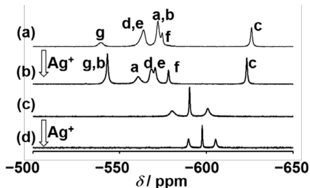
Fig. 7 ^{51}\text{V} NMR spectra of (a) closed-V12 , (b) closed-V12' , (c) opened-V12 and (d) opened-V12' . Signal assignment of closed-V12' based on ^{51}\text{V} - ^{51}\text{V} COSY NMR spectra were shown according to the labelling in Fig. 1.
