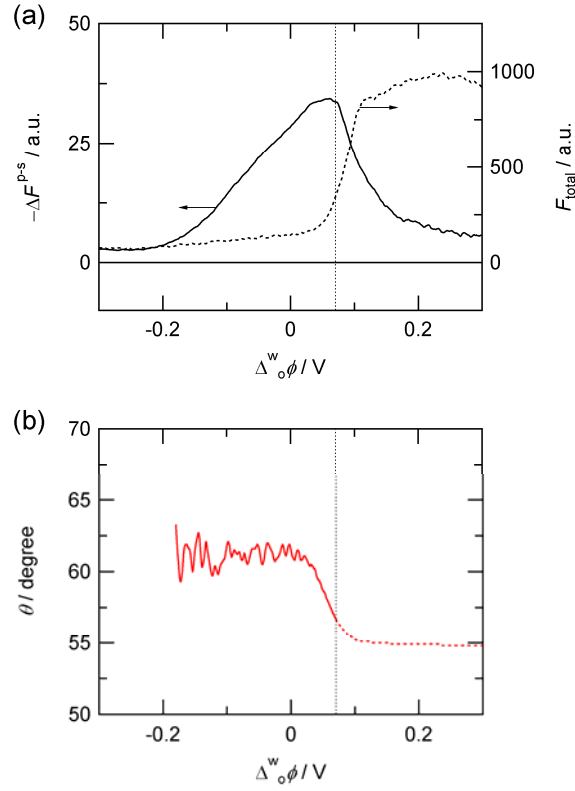
Figure 5. The potential dependence of (a) PM-TIRF responses ( \Delta F^{P-s} ) (solid) and F_{\text{total}} (dashed) and (b) the orientation angles ( \theta ) estimated from eqs. 6, 8 and 9 for \text{H}_2\text{TMPyP}^{4+} system. The potential sweep rate was 5 \text{ mV s}^{-1} . The fluorescence intensity was detected at 660 nm. The vertical dotted lines depict \Delta_o^w \phi_{\text{H}_2\text{TMPyP}^{4+}}^{\circ'} = 0.07 \text{ V} .
