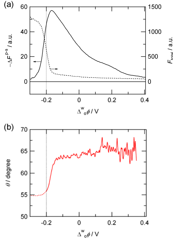
Figure 6. The potential dependence of (a) PM-TIRF responses ( \Delta F^{p-s} ) (solid) and F_{total} (dashed) and (b) the orientation angles ( \theta ) estimated from eqs. 6, 8 and 9 for H_2TPPS^{4-} system. The potential sweep rate was 5 \text{ mV s}^{-1} . The fluorescence intensity was detected at 649 nm. The vertical dotted lines depict \Delta_o^w \phi_{H_2TPPS^{4-}}^{s'} = -0.20 \text{ V} .
