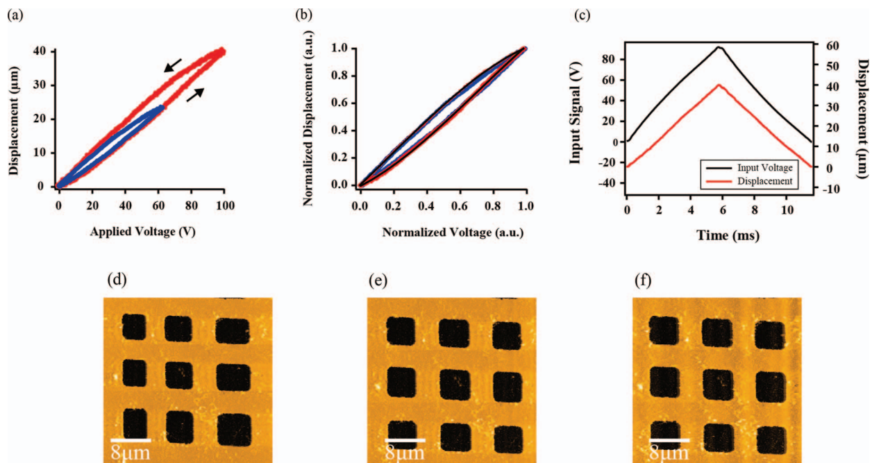
FIG. 3. Hysteresis of X-scanner and its compensation. (a) Hysteresis curves for two different ranges (blue line, 24 \mu\text{m} ; red line, 40 \mu\text{m} ). (b) Hysteresis curves normalized with regard to both displacement and voltage. Black line shows a fitting curve with fourth-order polynomials. (c) Driving signal of 85 Hz with a triangular wave form modified by open-loop compensation for hysteresis (black line) and corresponding displacement (red line). Here, hysteresis compensation was applied to a triangular wave form modified by inverse compensation. (d) AFM image of a test grating sample with a pitch of 10 \mu\text{m} obtained without hysteresis compensation (imaging rate, 7 s/frame; pixels, 256 \times 256 ). (e) AFM image of the same grating sample obtained using hysteresis compensation (imaging rate, 7 s/frame; pixels, 256 \times 256 ). (f) AFM image of the same grating sample obtained using hysteresis compensation (imaging rate, 3 s/frame; pixels, 256 \times 256 ).
