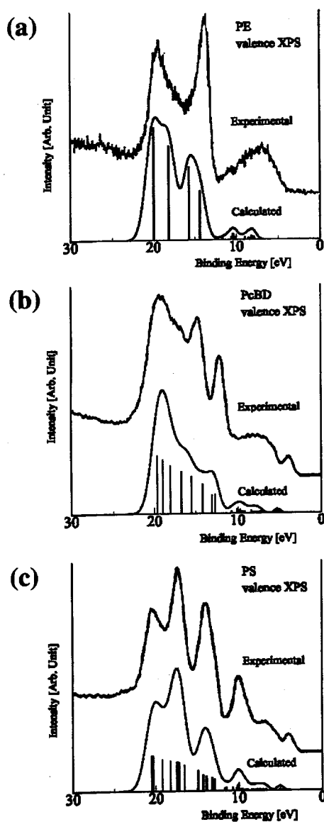
Fig. 1 Simulated valence X-ray photoelectron spectra of three polymers with the experimental spectra, (a) PE; (b) PcBD; (c) PS.
