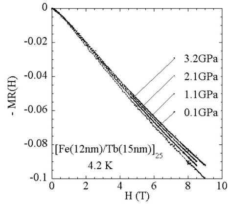
FIG. 3. MR curve of [\text{Fe}(12 \text{ nm})/\text{Tb}(15 \text{ nm})]_{25} at 4.2 K as a function of the magnetic field applied parallel on the plane. The value of MR is obtained by using Eq. (1).
