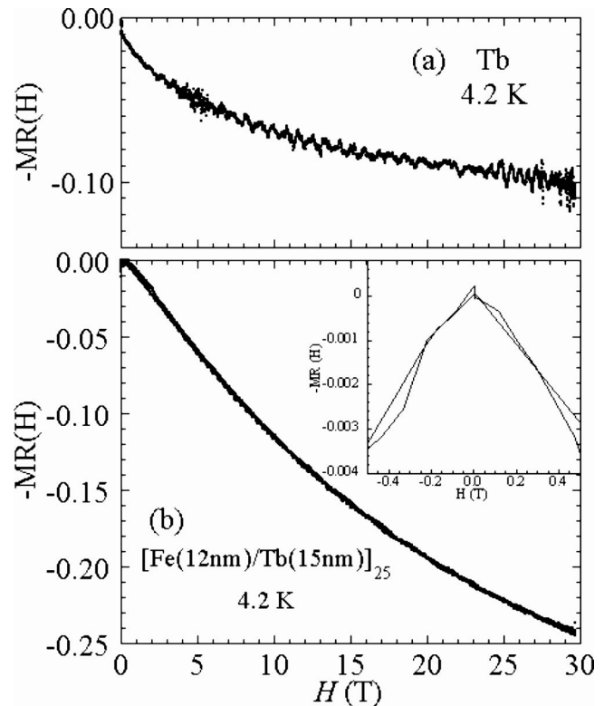
FIG. 1. The MR curves of (a) Tb at 4.2 K and (b) [\text{Fe}(12 \text{ nm})/\text{Tb}(15 \text{ nm})]_{25} as a function of the magnetic field applied parallel on the plane. Inset shows the MR curve of Fe/Tb from -0.5 to 0.5 T.
