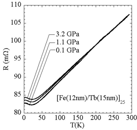
FIG. 2. The electrical resistance of [\text{Fe}(12 \text{ nm})/\text{Tb}(15 \text{ nm})]_{25} as a function of the temperature at several pressures.
