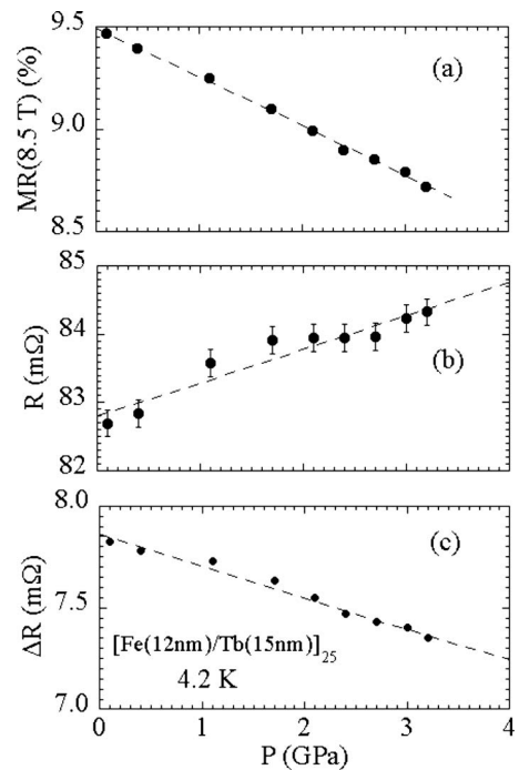
FIG. 4. Pressure dependences of (a) \text{MR}(8.5 \text{ T}) , (b) the electrical resistance at 0 T, and (c) the MR \Delta R at 8.5 T of [\text{Fe}(12 \text{ nm})/\text{Tb}(15 \text{ nm})]_{25} at 4.2 K.
