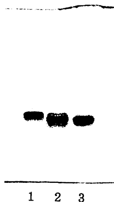
Fig. 3. Polyacrylamide gel electrophoresis of isolated TNBS-modified salicylate hydroxylase. Lane 1, native enzyme; lane 2, modified enzyme before purification; and lane 3, modified enzyme after purification. The electrophoresis was carried out on 7.5% polyacrylamide gel (26) and proteins were stained with Coomassie Blue.
