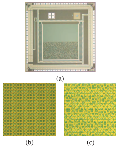
Fig. 6. Fabricated CMOS image sensor with pseudorandom pixel placement.(a)whole circuit, (b)part of lattice pixel plain, and (c)part of pseudorandom pixel plain.
