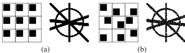
Fig. 3. Examples of the effect of directional dependency in two types of pixel placements. (Left: example of pixel placement. Right: represented image.) (a) Image obtained with conventional lattice pixel placement, (b) image obtained with pseudorandom pixel placement. Pseudorandom placement reduces the effect below the level of perception.
