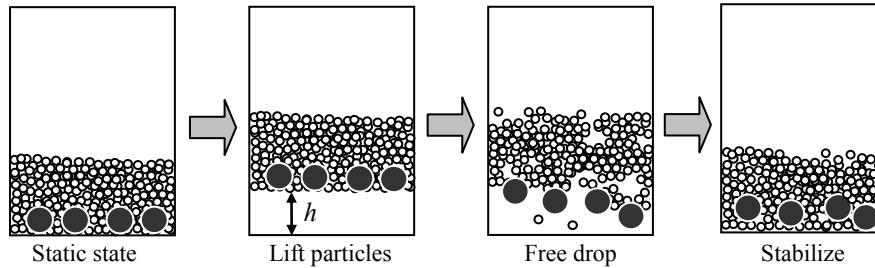
Fig. 10. Modeling of excitation process
