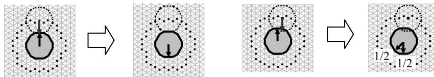
Fig. 9. Examples of rule for medium particle collision
