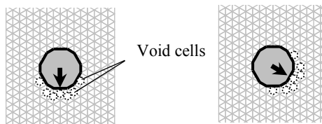
Fig. 8. Examples of rule for medium particle movement, collision between particles.
