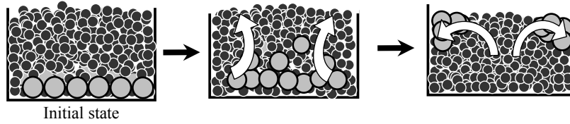
Fig. 4. Schematic of segregation process
