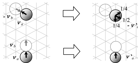
Fig. 7. Examples of rule for small particle collision
