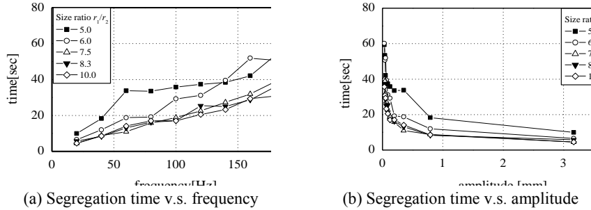
Fig. 2. Segregation time observed in experiment
