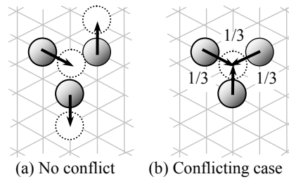
Fig. 6. Examples of rule for small particle movement
