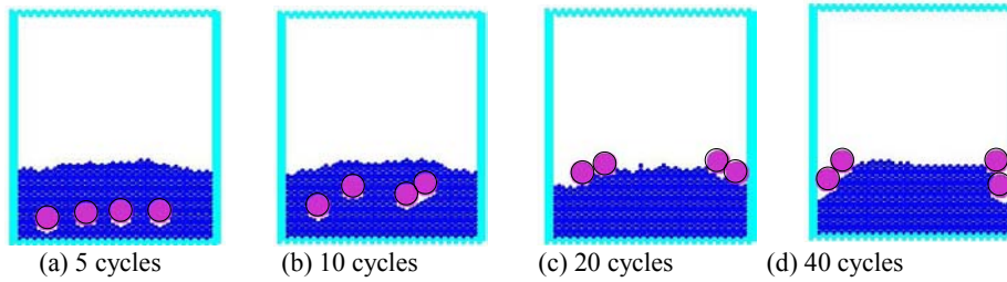
Fig. 14. Simulation result of small-medium particle segregation
