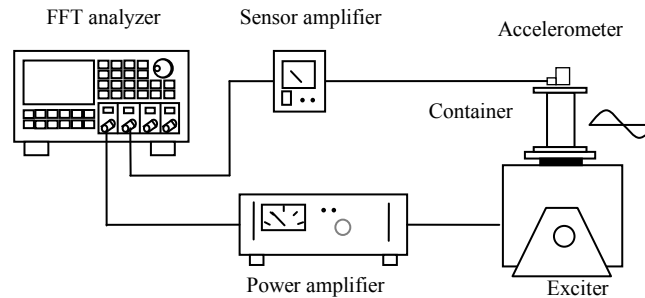
Fig. 1. Experimental setup of size-segregation of grains.
