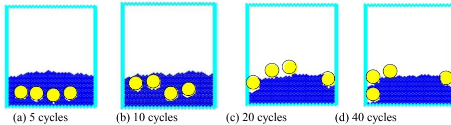
Fig. 15. Simulation result of small-large particle segregation
