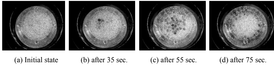
Fig. 3. Segregation process of larger particles
