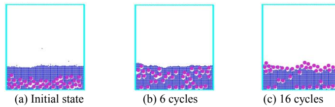
Fig. 12. Simulation result of small-medium particle segregation (2500 small, 40 medium particles)
