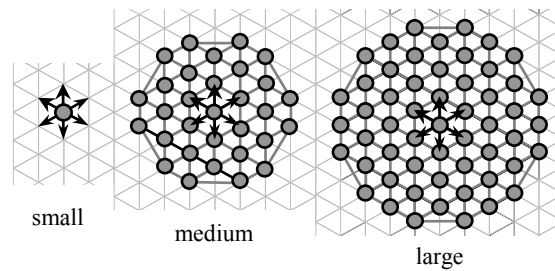
Fig. 5. Space segmentation and particle definition
