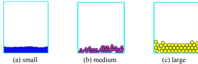
Fig. 11. Accumulation of homogeneous grains
