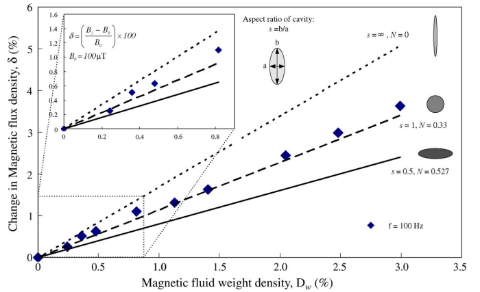
Fig. 6. Estimation of magnetic fluid weight density in tray with embedded cavities.
