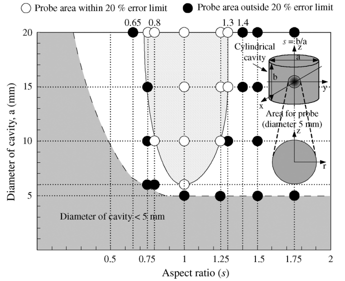
Fig. 3. Condition for cavity for 20% error inside 5-mm spherical area.
