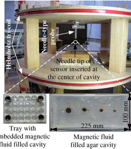
Fig. 5. Experimental setup.
