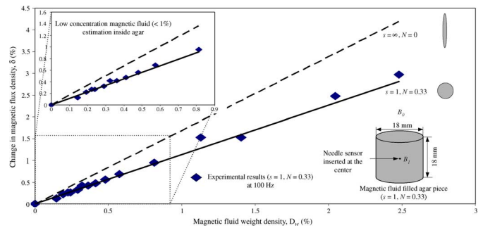
Fig. 8. Estimation of magnetic fluid weight density inside agar.
