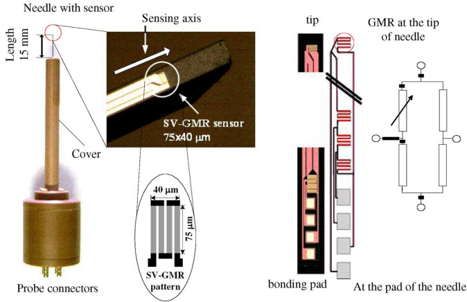
Fig. 4. Fabricated needle-type GMR sensor.
