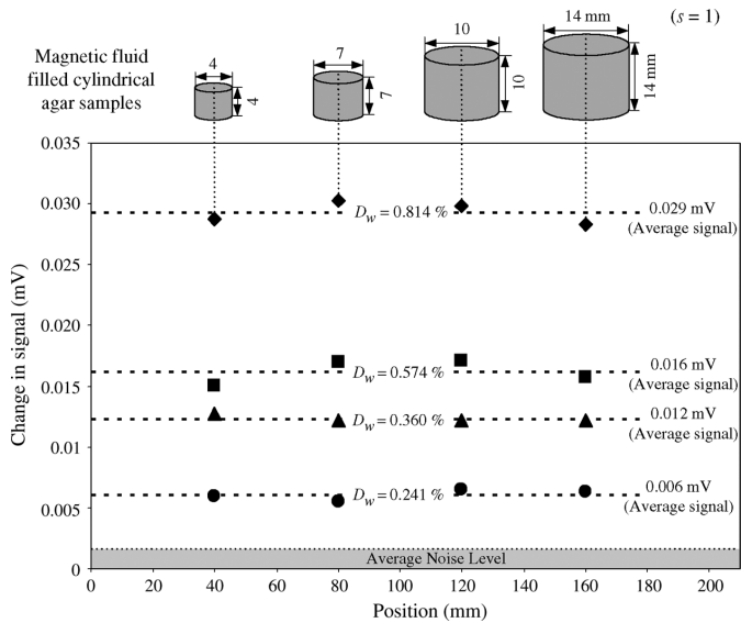
Fig. 7. Detection of magnetic fluid inside agar.
