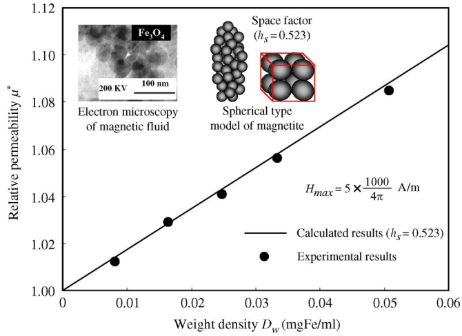
Fig. 1. Relative permeability as a function of weight density ( H_0 = 100 A/m), assuming space factor h_s , of 0.523.
