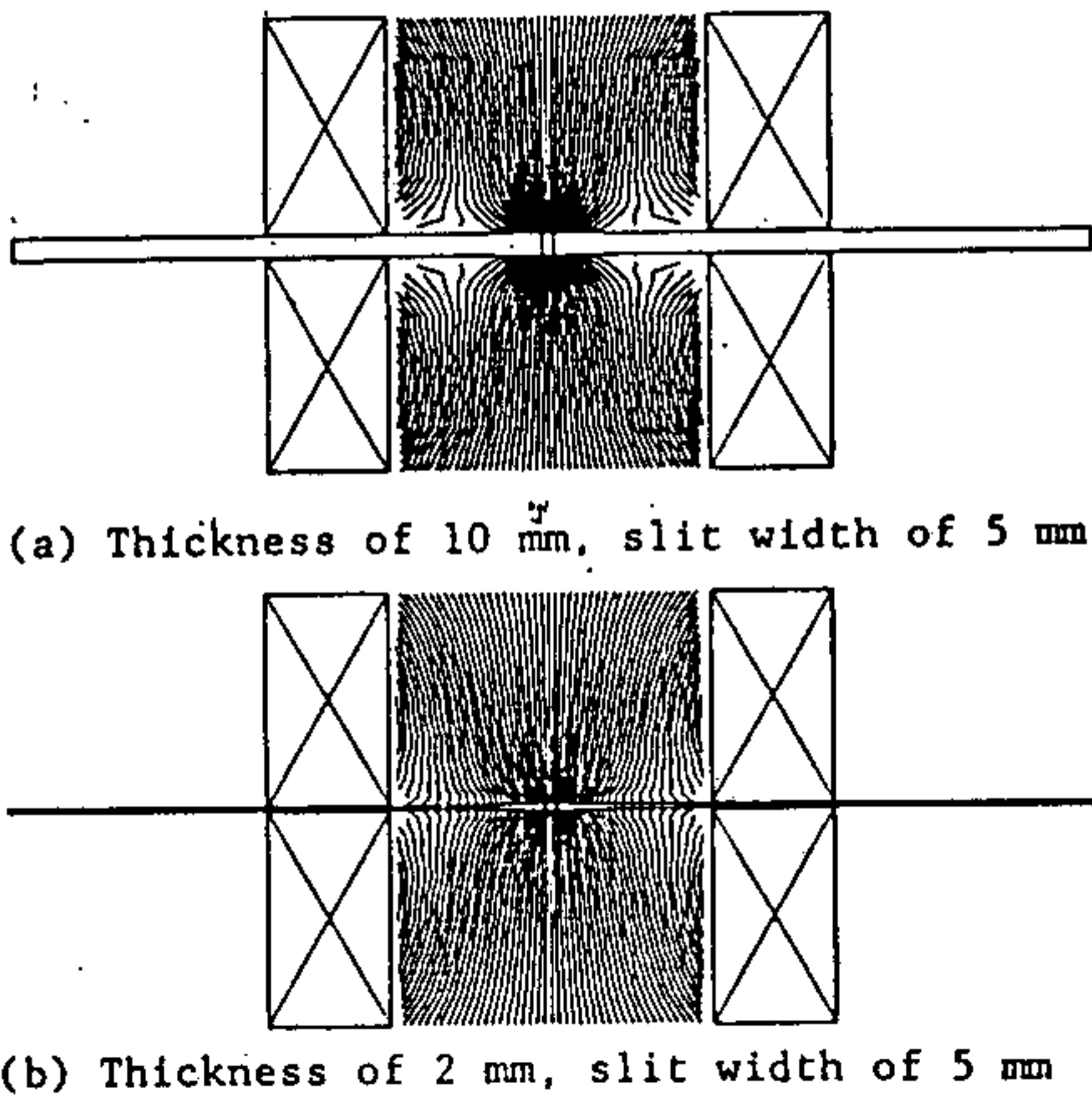
Fig.5 Flux distribution
