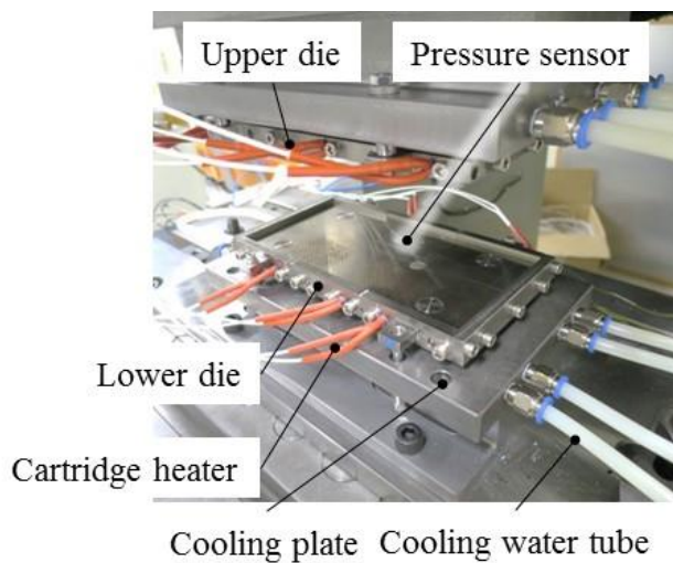
Fig. 4 Appearance of the die
