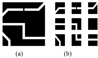
Fig. 2. (a) A typical PCB pattern sheet. (b) The pattern is disassembled to nine basic parts.
