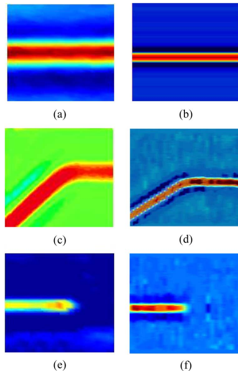
Fig. 6. (a), (c), and (e) are the images obtained from experiment and (b), (d), and (f) are the images produced by the base-model method. Scanning was done in an up-down direction.
