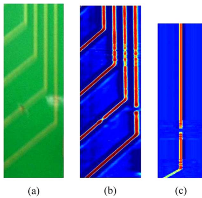
Fig. 5. (a) Photo of a real PCB. (b) Image of the PCB obtained by experiment after applying image processing technique. (c) Image obtained by base-model method for a small part of the PCB.
