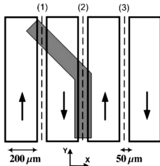
Fig. 3. Top view of 3D FEM simulation of the problem. An open-elbow PCB basic part, 100 \mu\text{m} width, shown in gray is set 50 \mu\text{m} under four legs of Meander coil.
