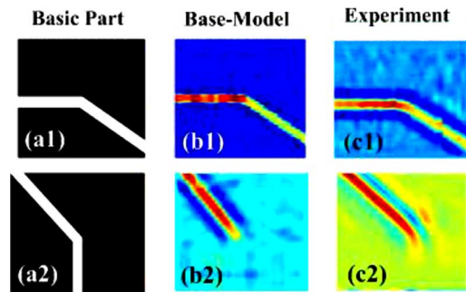
Fig. 4. (a1), (a2) Basic parts obtained after disassembling. (b1), (b2) Base-model results of scanning simulation based on 3D FEM analysis. (c1), (c2) Experimental results of the same pattern PCB, notice that the scanning direction is from left to right in the horizontal direction.
