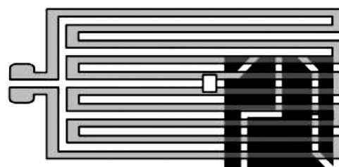
Fig. 1. A Meander-type coil is shown above a PCB while a GMR sensor is set at the midpoint of the coil.
