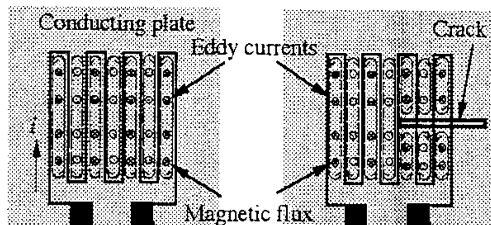
(a) Pattern of eddy currents when there is no crack (b) Pattern of eddy currents when a crack exists
