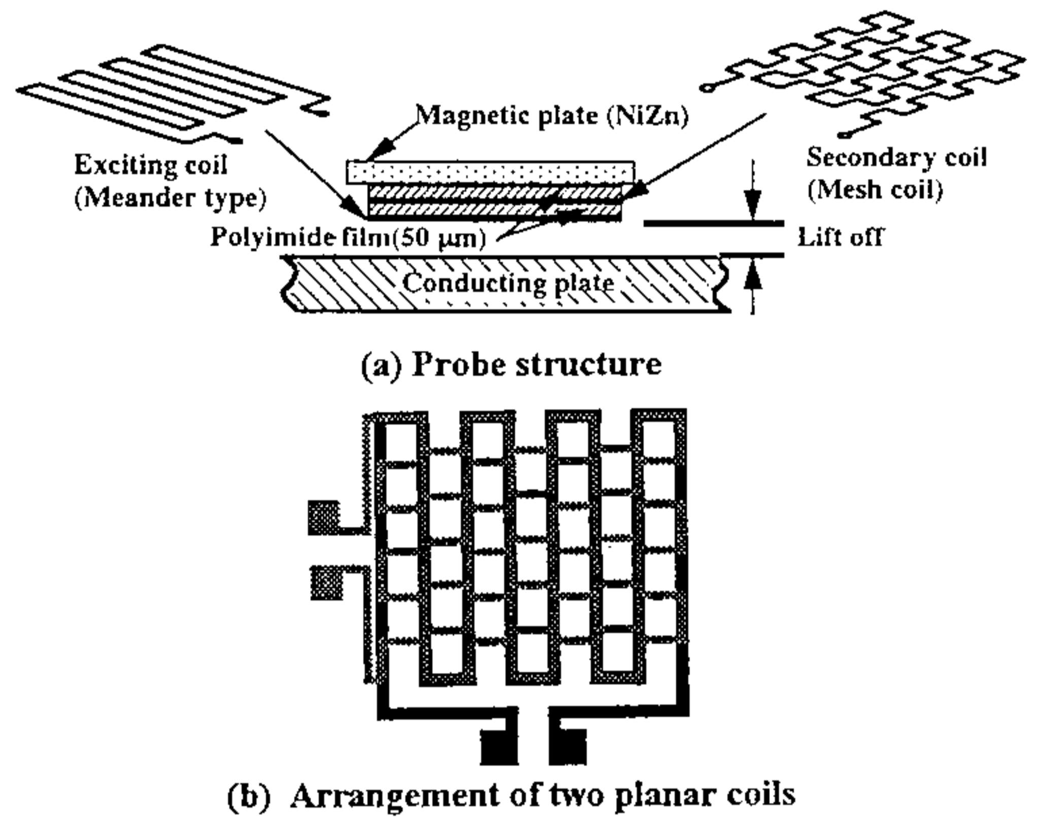
Fig.1 ECT Probe Composed of Two Kinds of Planar Coils
