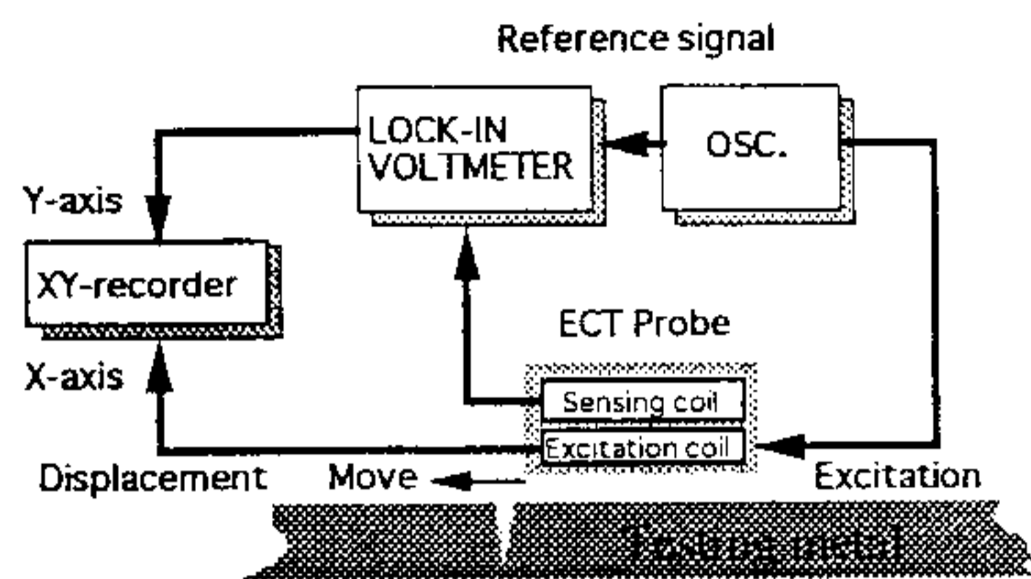
Fig. 4 Measurement System
