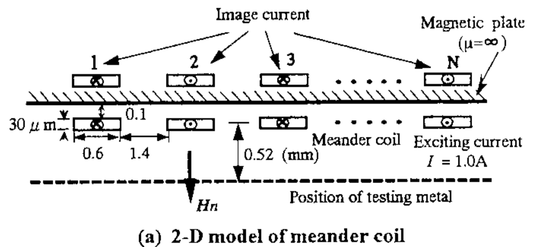
Fig.1 ECT Probe Composed of Two Kinds of Planar Coils
