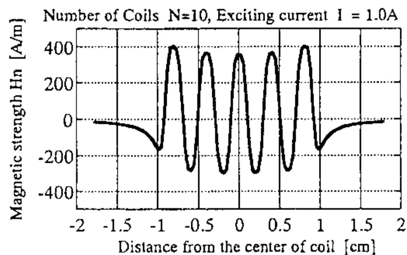
(b) Magnetic strength distribution with 0 distance coinciding with the centre of the meander coil
