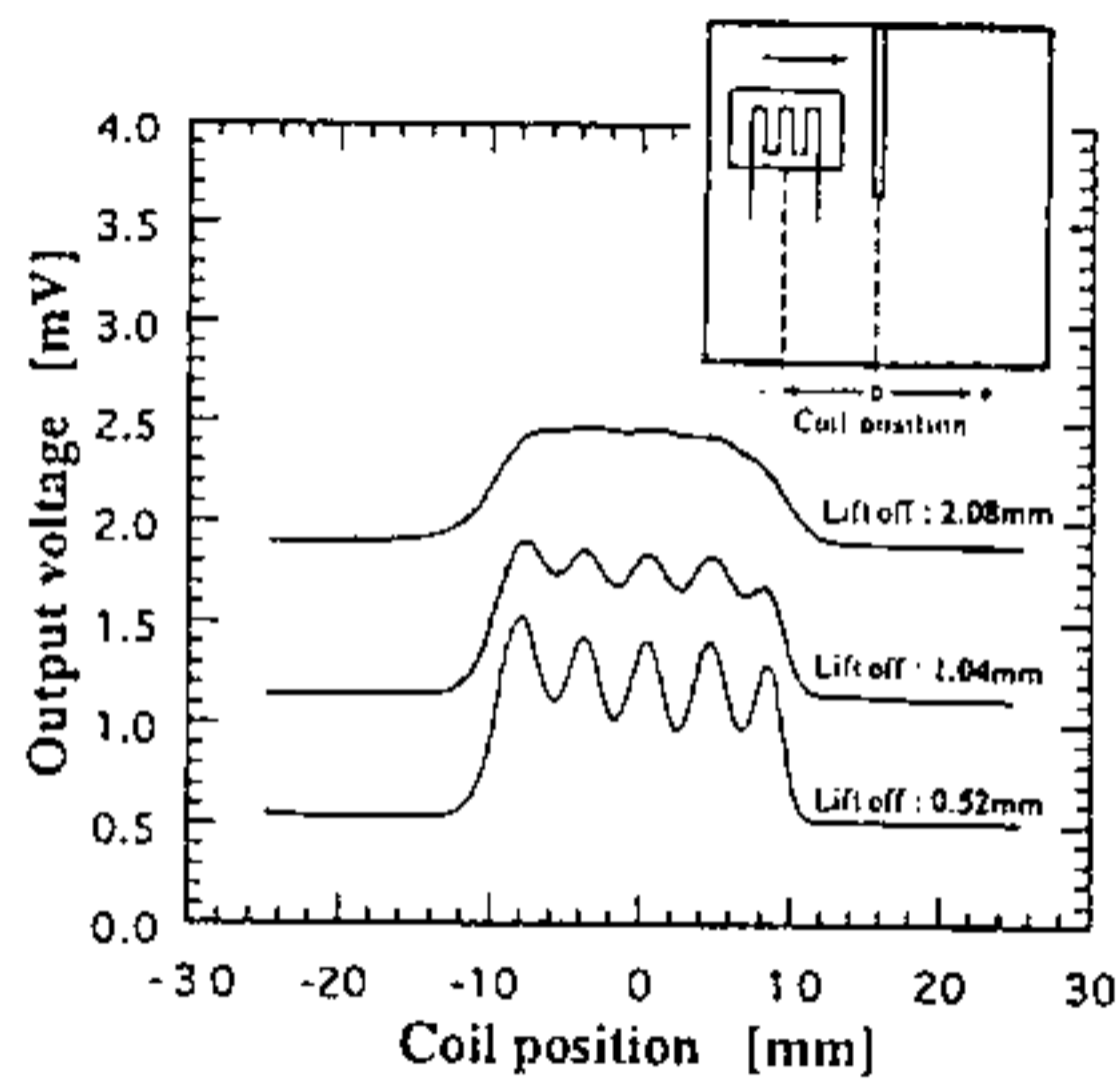
(a) Crack length parallel to the motion of the coil assembly
