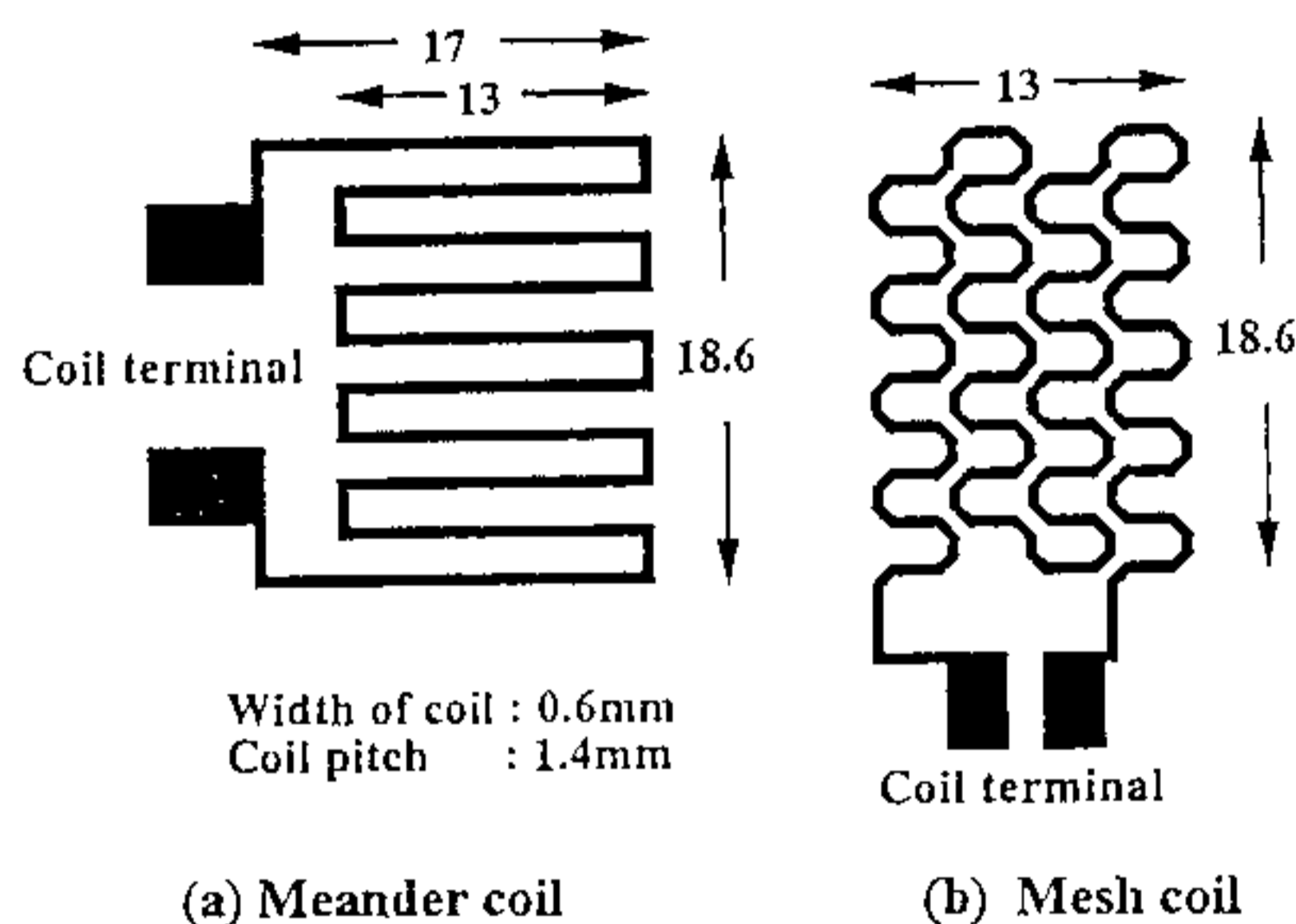
Fig. 5 Coil Pattern
