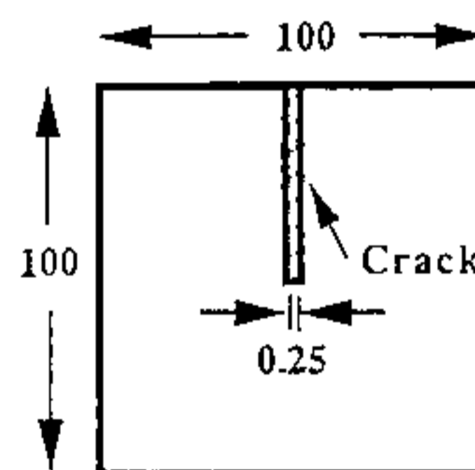
Fig. 6 Placement of a Crack in a Copper Plate
