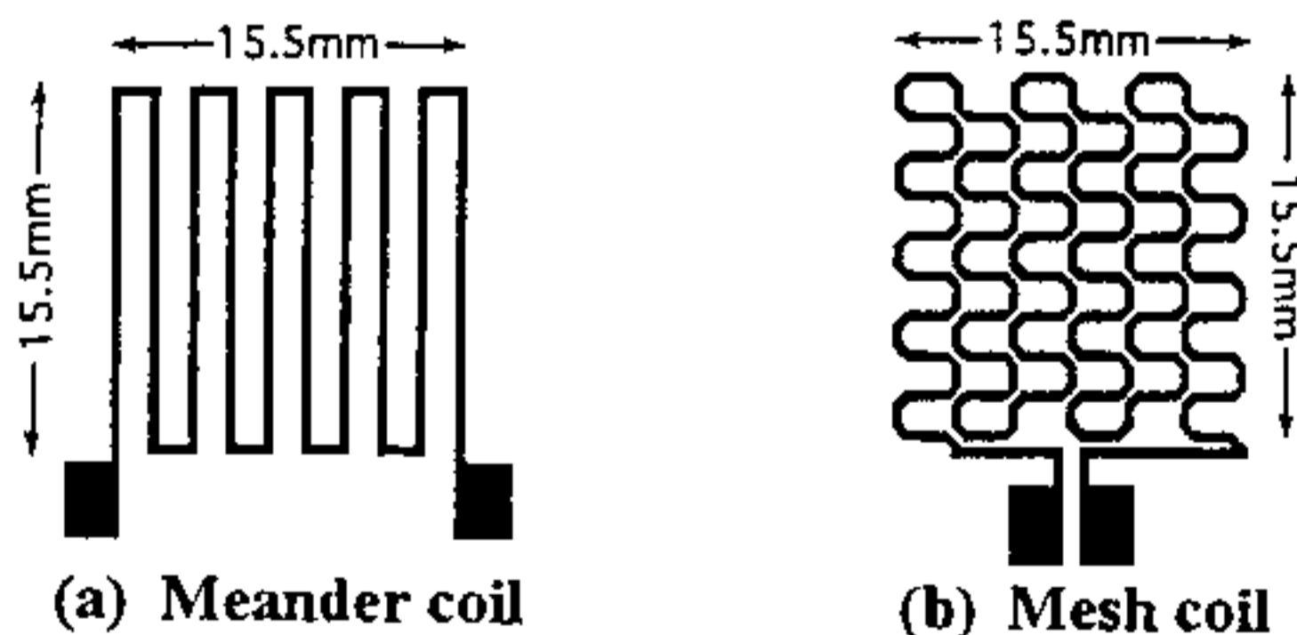
Fig. 9 Coil Structure
