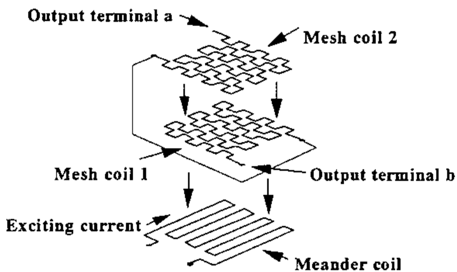
Fig. 8 Two Mesh Coil Configuration
