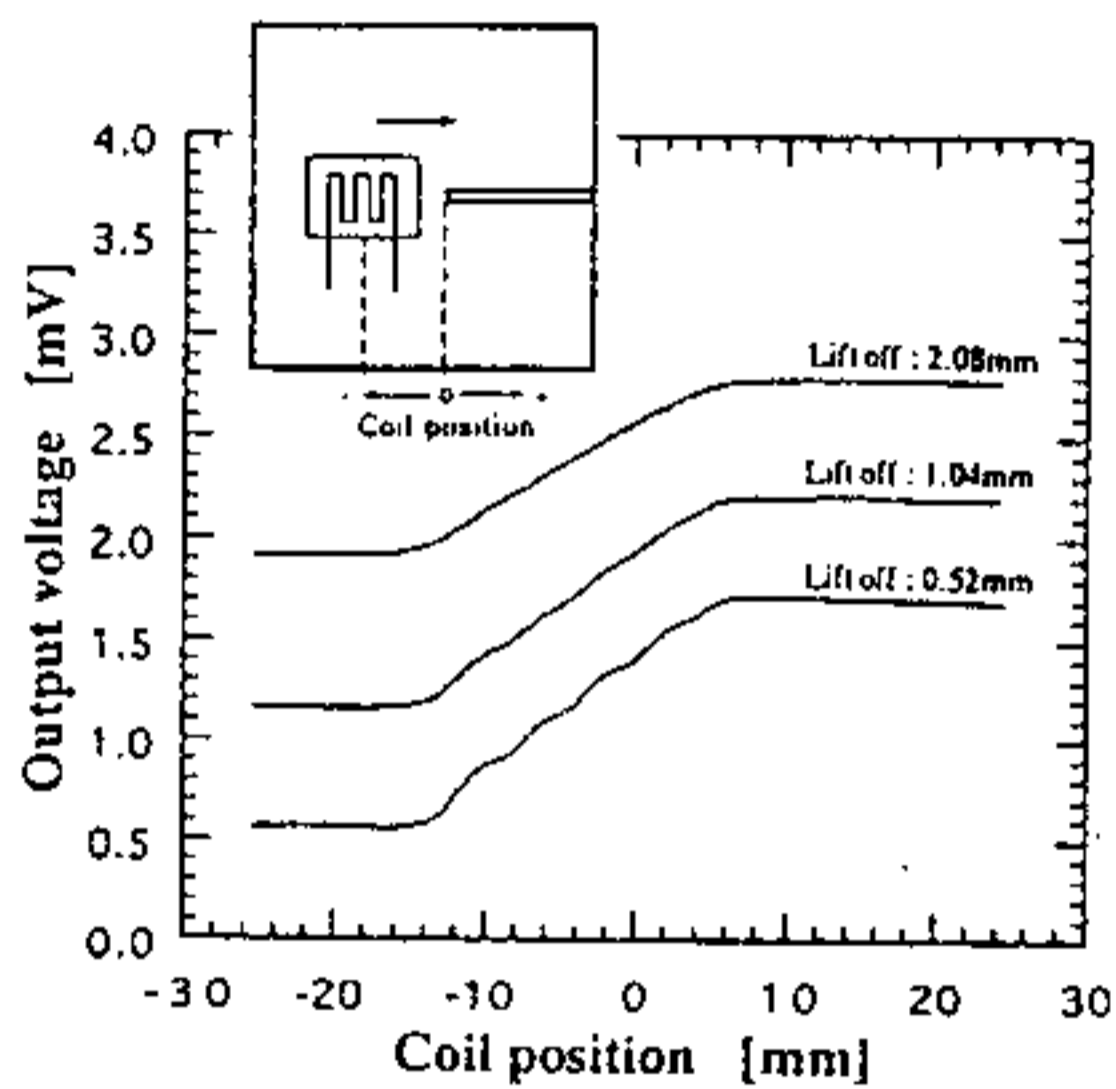
(b) Crack length perpendicular to the direction in motion of the coil assembly
