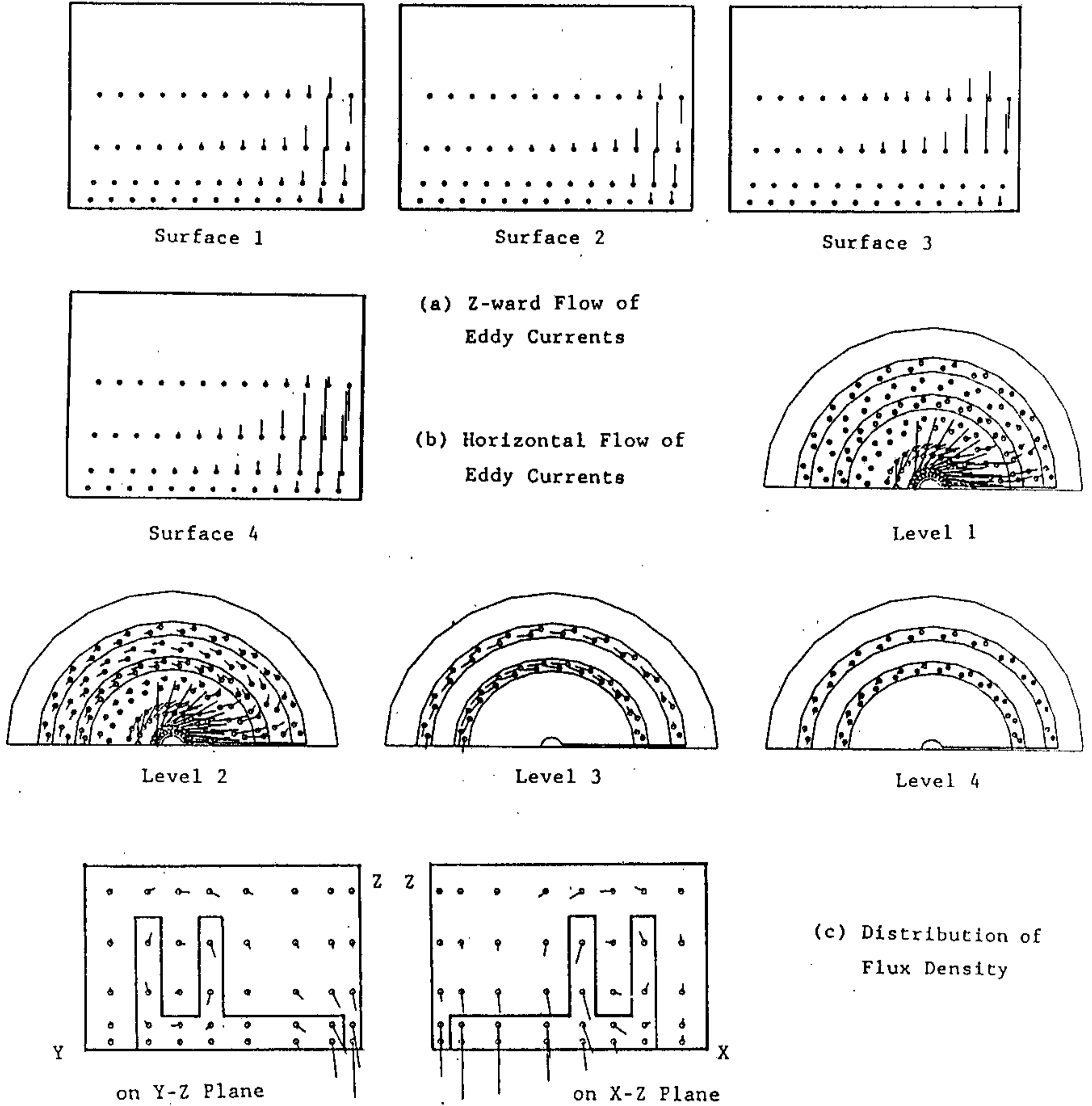
Fig.5 Computed Results for Case 2
