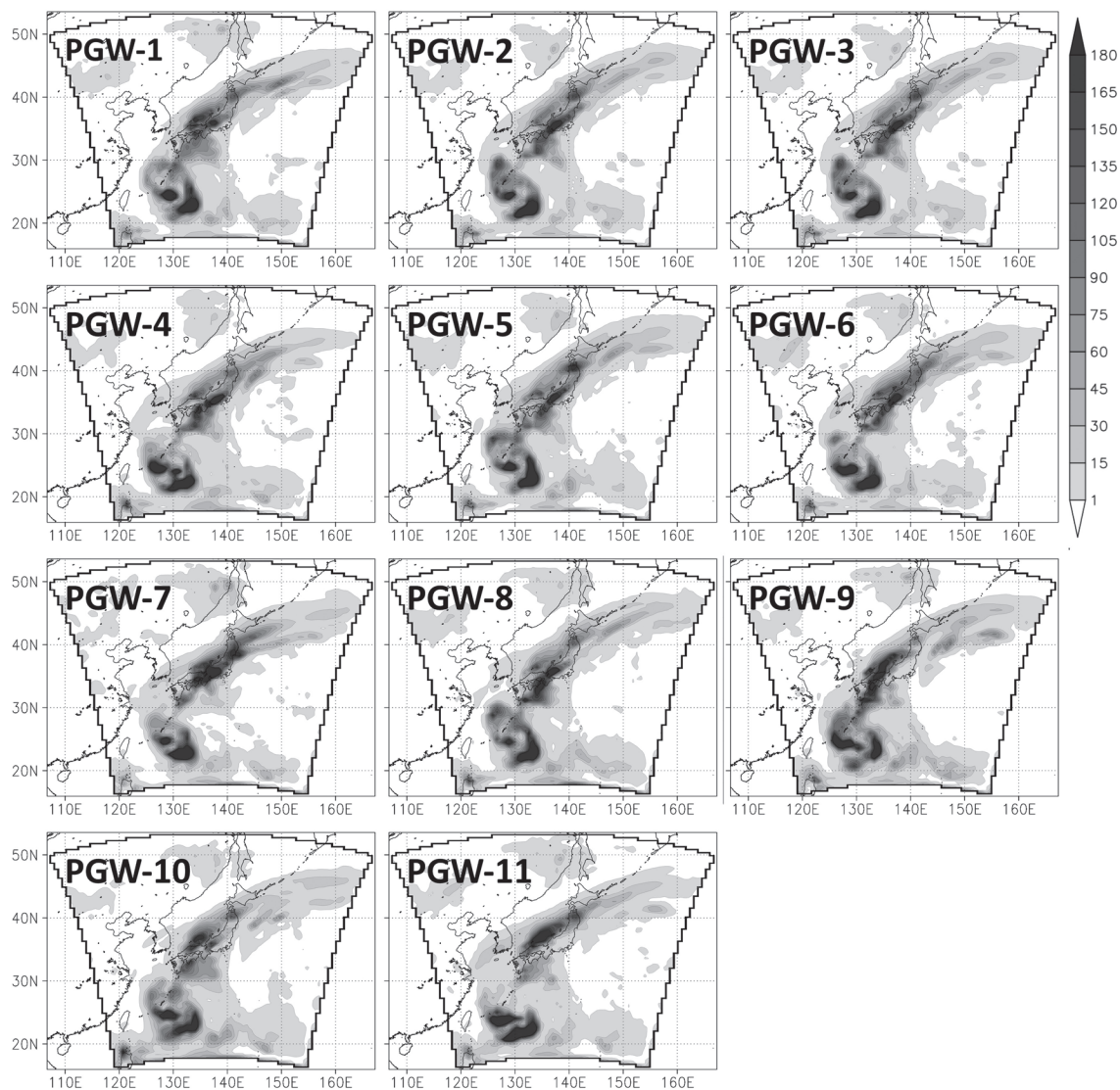
Fig. 5. Spatial distributions of total precipitation in D01 from 21 JST 10 September to 21 JST 12 September for ENS1 of 11 PGW runs. Color bar shows rainfall (mm).
