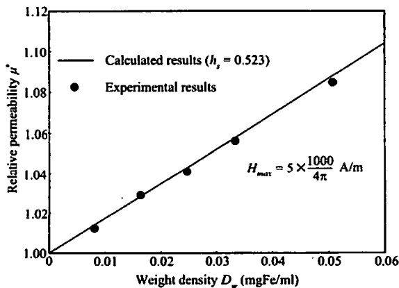
Fig. 2 Relationship between relative permeability and magnetic fluid weight density.
