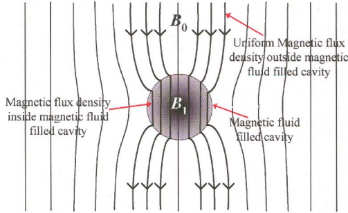
FIGURE 7. Model for estimating the volume of magnetite. The magnetic flux density inside the imbedded cavity is measured by magnetic sensor.
