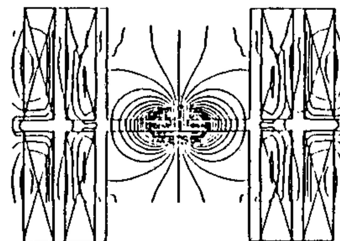
FIG. 5. Equivalent-potential lines.
