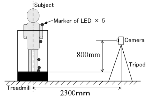
Fig.4. Walking measurement system
