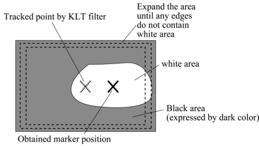
Fig. 7. Estimated marker position based on the tracked point by KLT filter
