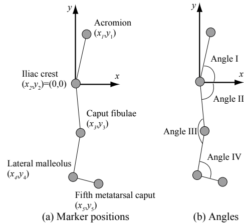
Fig.5. Coordinate frame, marker positions, and angles
