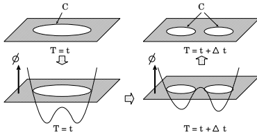
Fig. 1. Concept Map of the Level Set Method.
