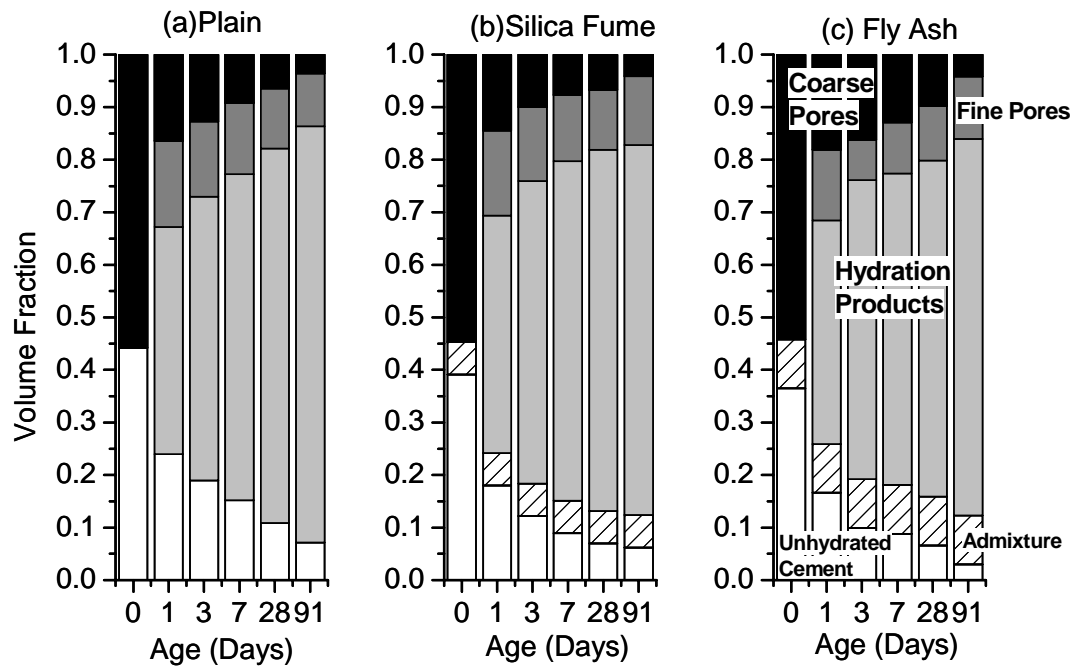
Figure 6 Volume fractions of constituent phases in w/c ratio 0.4 cement pastes with a mineral admixture Coarse pores: >0.2\mu\text{m} Fine pores: 0.2\mu\text{m}-2.6\text{nm}
