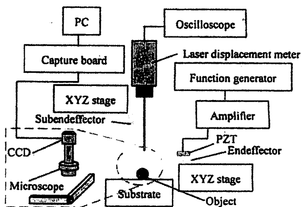
Fig. 2 Overview of the experimental setup
