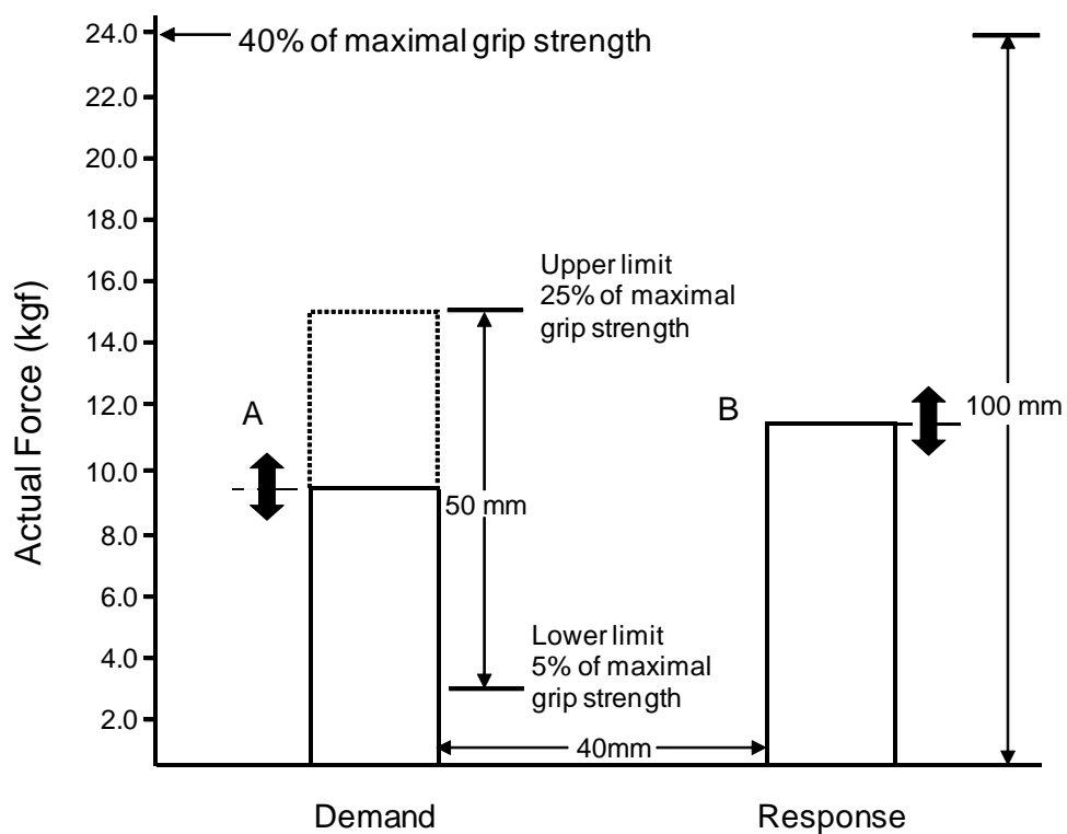
Figure. 2. Bar chart display (100 mm X 140 mm) of demand value. Bar chart display (100 mm X 140 mm) of demand value. Left bar (A) shows the demand value and right bar (B) is the exertion value of grip strength. The test was to fit line B (exertion value of grip strength) to line A (demand value), which varied in a span of 50 mm on the display. The test time was 40 sec for each trial. The controlled force exertion was calculated using the data from 25 sec of the trial following the initial 15 sec of the 40-sec period. Actual force was shown on the display, right.
