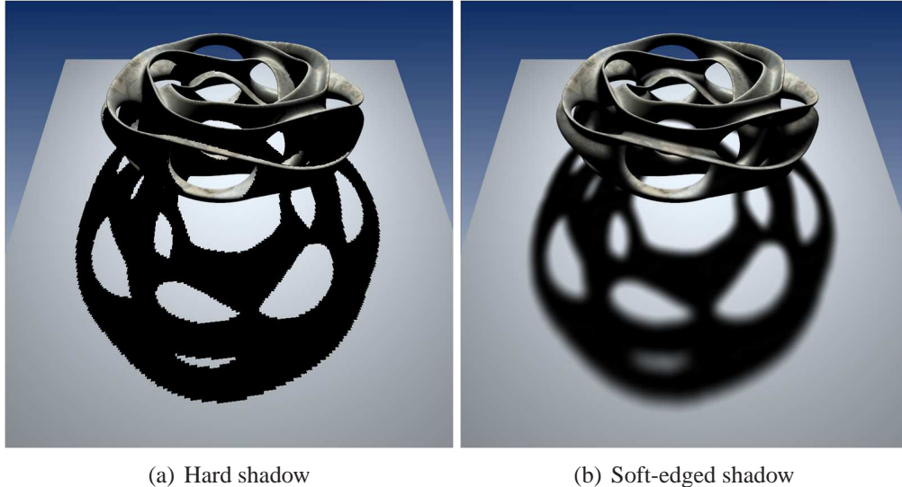
Figure 2.5: The illustration of hard shadow and soft-edged shadow.
