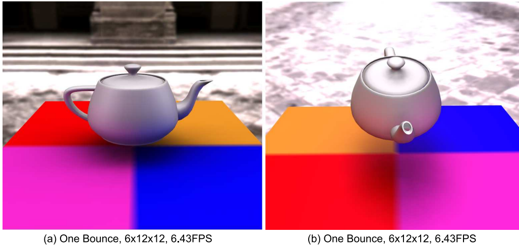
Figure 4.1: Teapot with indirect lighting (3878 vertices).
