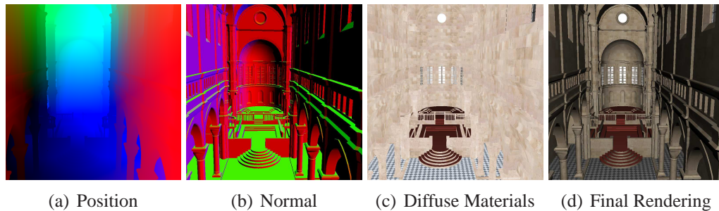
Figure 2.15: Deferred shading with G-buffers.
