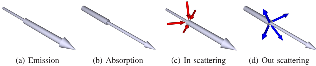
Figure 2.11: Interaction of light in a participating medium.
