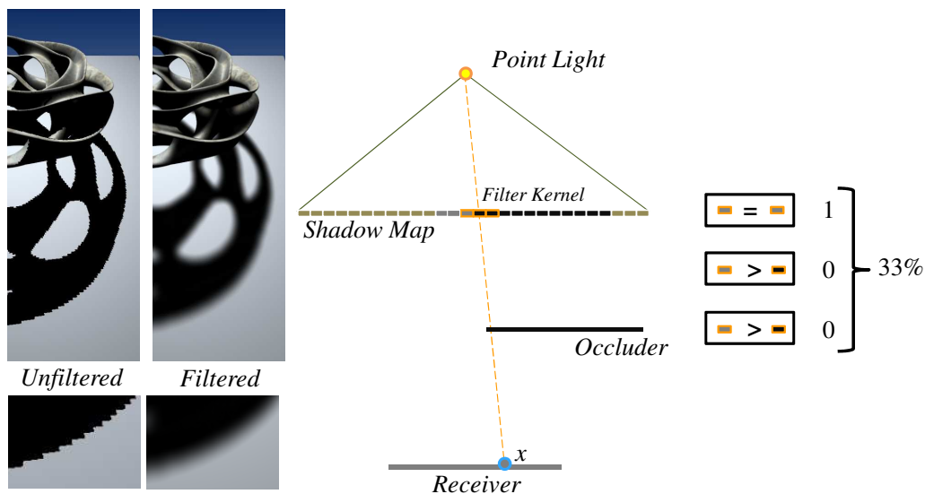
Figure 2.8: The illustration of percentage closer filtering shadow mapping.
