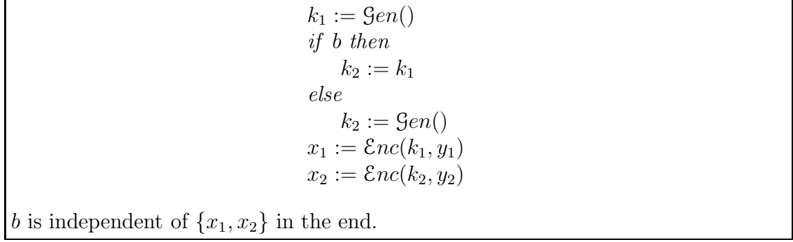
Figure 4.9: The example program
