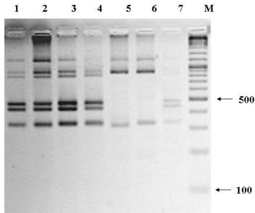
Figure 4. The nested R16F2n/R16R2 amplified fragment digested with KpnI .
