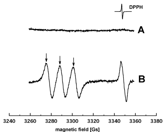
Figure 1. In vitro spin trapping of • NO by Fe(DTCS) 2 .
