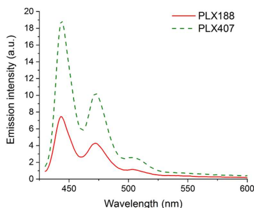
Figure 12. Emission spectra of perylene solubilized by either Poloxamer ® 188 or Poloxamer ® 407 solution ( \lambda_{\text{ex}} = 405 nm).
