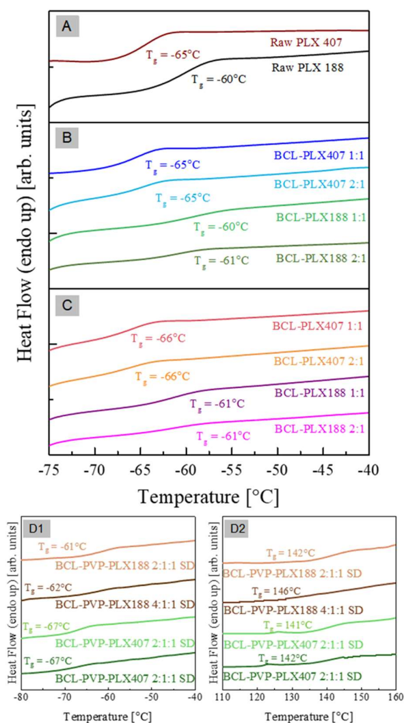
Figure 8. The zoomed fragment of DSC thermograms presented in the Figure 7 of raw bicalutamide and poloxamers (A), binary systems containing bicalutamide and either PLX188 or PLX407 obtained using evaporation method (B) and spray drying (C), and ternary, spray-dried, systems containing BCL, poloxamer, and PVP (D1,D2).
