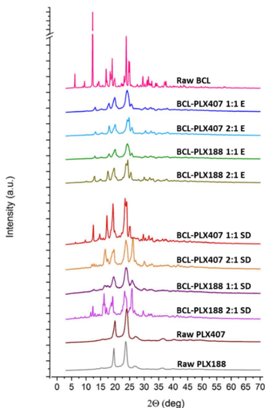
Figure 4. X-ray diffraction patterns of binary systems containing bicalutamide and either PLX 188 or PLX 407 (1:1 and 2:1 wt. ratio) obtained using evaporation technique (E) and spray drying (SD).
