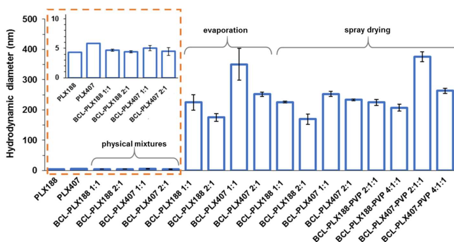
Figure 10. Hydrodynamic diameters of aggregates formed in aqueous solutions of poloxamers, physical mixtures, and binary systems obtained using either the evaporation method or spray drying. Insert: zoomed data corresponding to raw PLXs and physical mixtures.
