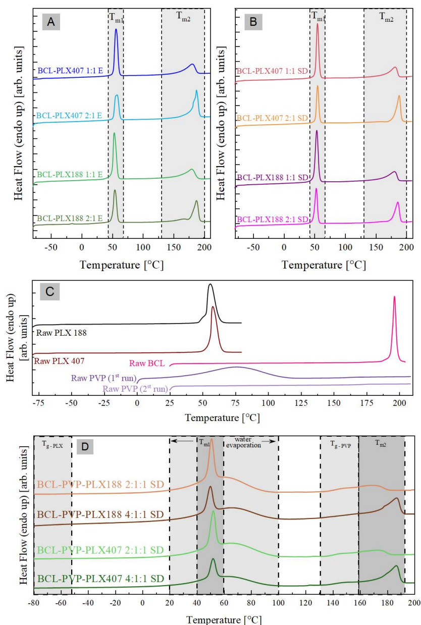
Figure 7. The DSC thermograms of: binary systems containing bicalutamide and either PLX188 or PLX407 obtained using the evaporation method (A) and spray drying (B), raw bicalutamide and polymers (C), and ternary spray-dried systems containing BCL, poloxamer, and PVP (D).
