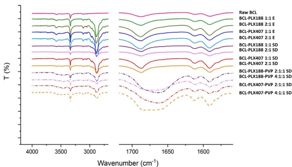
Figure 6. FTIR spectra of raw bicalutamide and binary and ternary solid dispersions.
