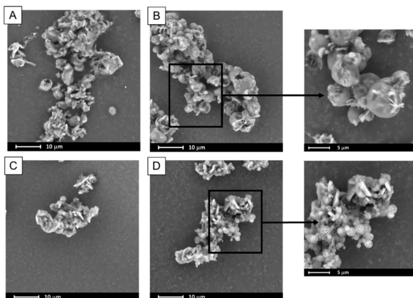
Figure 3. SEM images of ternary systems containing bicalutamide, PVP and either PLX188 in 4:1:1 (A) and 2:1:1 (B) wt. ratio or PLX407 in 4:1:1 (C) and 2:1:1 (D) wt. ratio obtained using spray drying.
