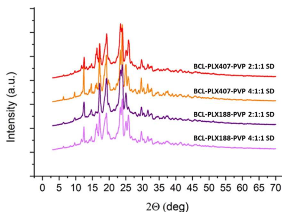
Figure 5. X-ray diffraction patterns of ternary systems containing bicalutamide, PVP, and either PLX 188 or PLX 407 obtained by spray drying.
