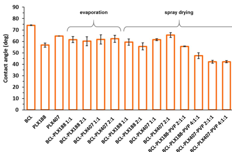
Figure 9. The values of contact angles of raw bicalutamide and poloxamers, binary and ternary systems containing bicalutamide, poloxamers, and PVP obtained using either evaporation method or spray drying.
