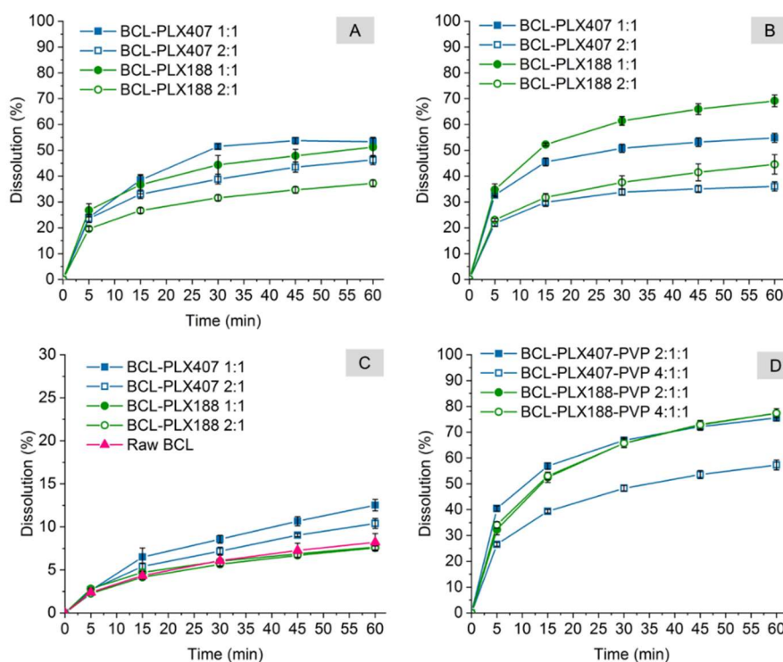
Figure 13. Dissolution of binary and ternary systems containing bicalutamide, poloxamers and PVP (in case of ternary systems) obtained using the evaporation technique (A), spray drying (B,D), and physical mixing (C).
