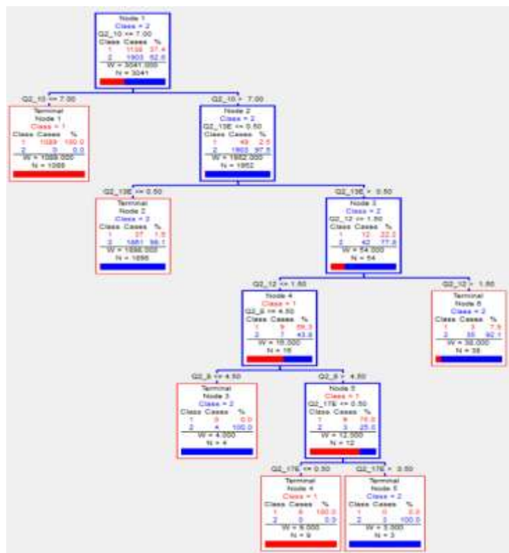
Fig-1: Decision Tree Using CART
