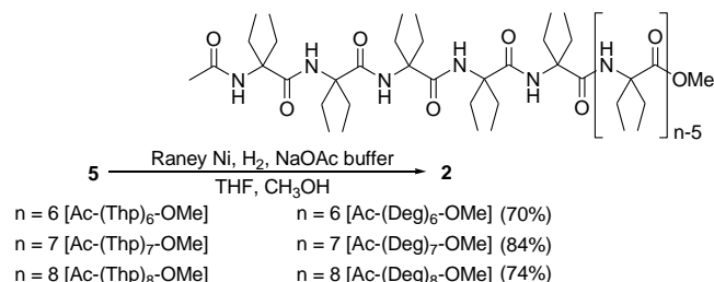
Figure 4. Synthesis of Ac-(Deg) n -OMe by Raney Ni desulfurization of Ac-(Thp) n -OMe.
